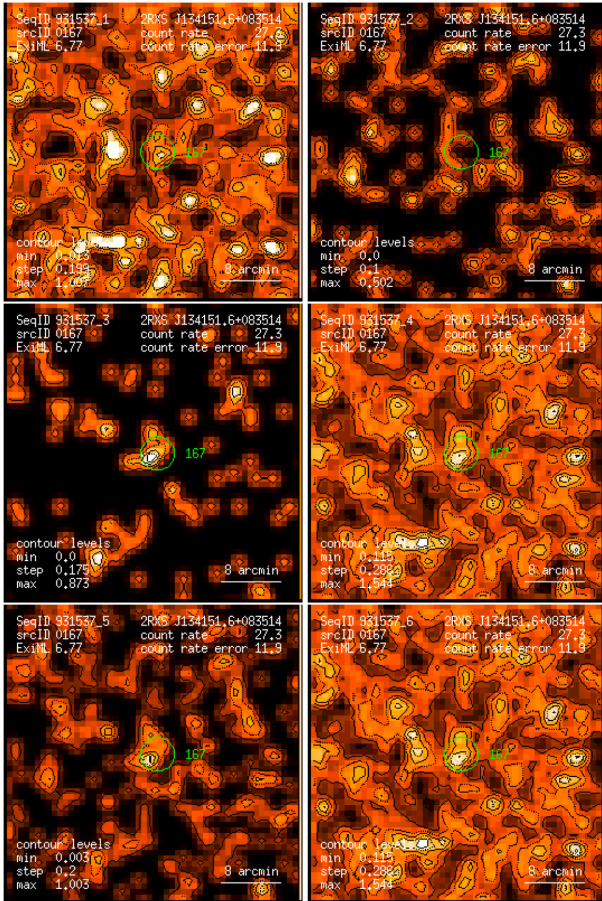
Figure 167: RASS 931537: detection 0167: band rate images, Gaussian filter: (1) PSPC channels 11 – 41, (2) 52 – 90, (3) 91 – 201, (4) 11 – 235, (5) 52 – 201, (6) 11 – 201. Broad band rates in counts/ks. Band rate contour levels in counts/ks/arcmin 2 .
