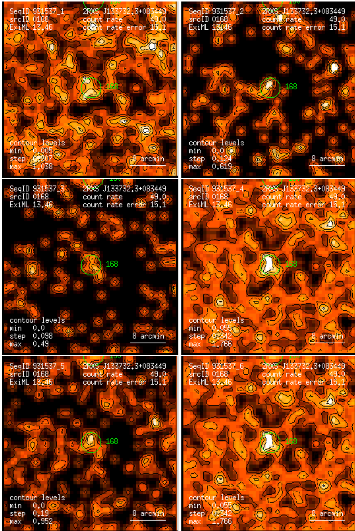
Figure 168: RASS 931537: detection 0168: band rate images, Gaussian filter: (1) PSPC channels 11 – 41, (2) 52 – 90, (3) 91 – 201, (4) 11 – 235, (5) 52 – 201, (6) 11 – 201. Broad band rates in counts/ks. Band rate contour levels in counts/ks/arcmin 2 .
