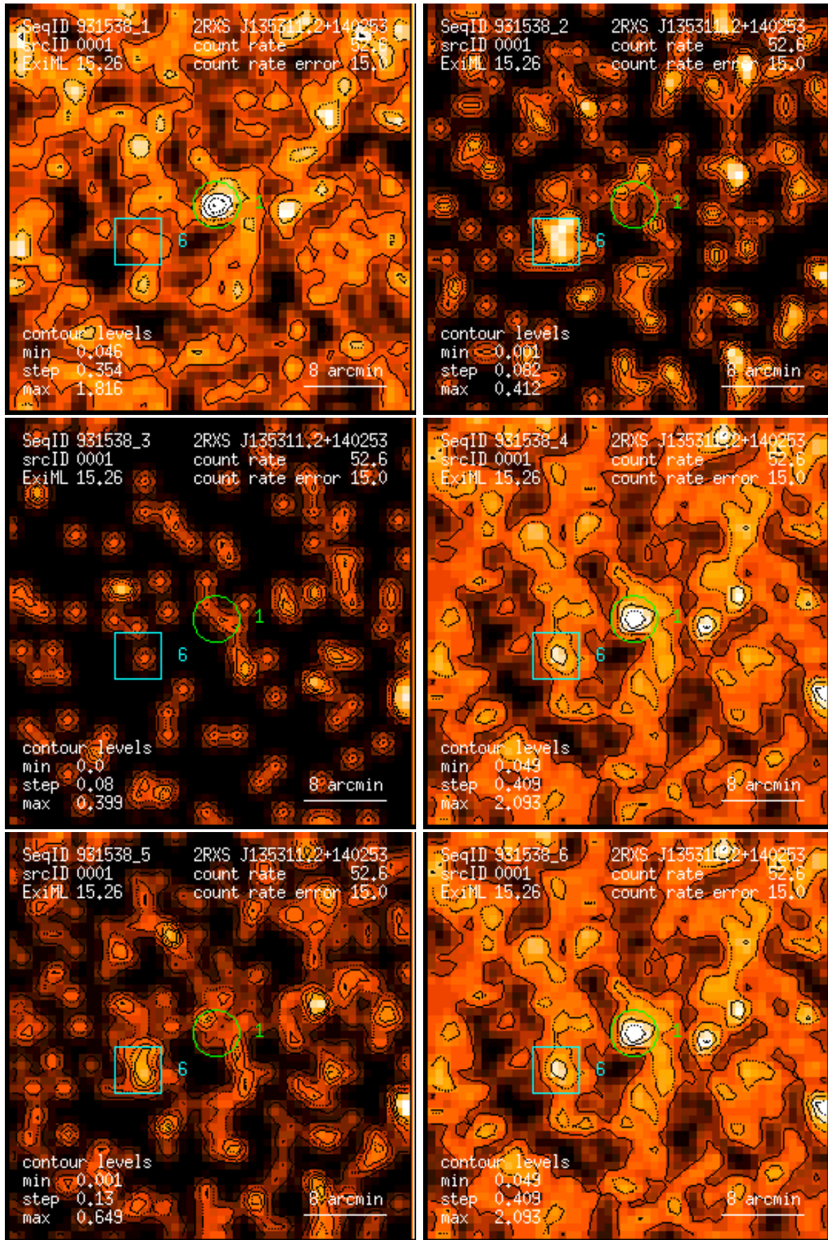
Figure 1: RASS 931538: detection 0001: band rate images, Gaussian filter: (1) PSPC channels 11 – 41, (2) 52 – 90, (3) 91 – 201, (4) 11 – 235, (5) 52 – 201, (6) 11 – 201. Broad band rates in counts/ks. Band rate contour levels in counts/ks/arcmin 2 .
