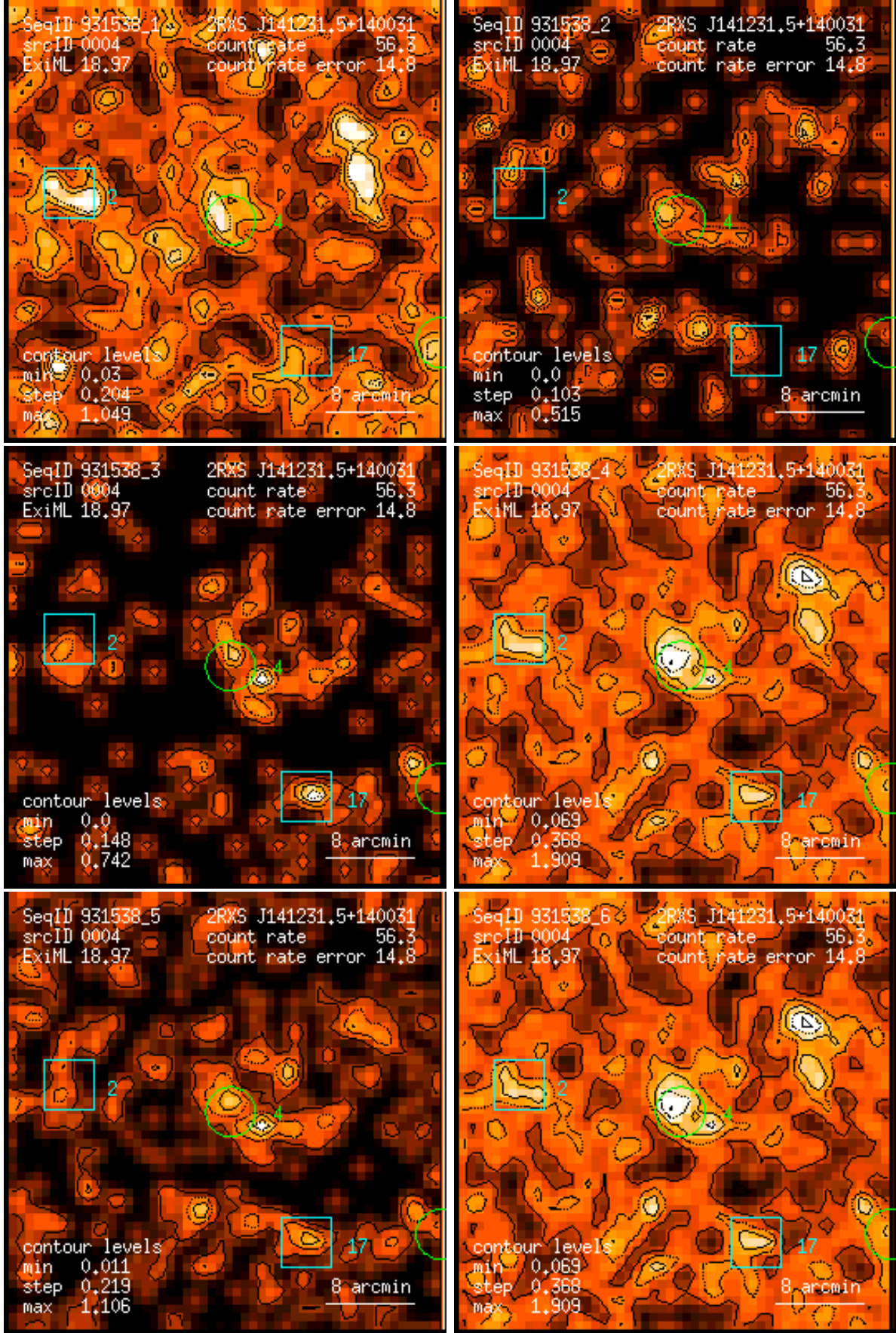
Figure 4: RASS 931538: detection 0004: band rate images, Gaussian filter: (1) PSPC channels 11 – 41, (2) 52 – 90, (3) 91 – 201, (4) 11 – 235, (5) 52 – 201, (6) 11 – 201. Broad band rates in counts/ks. Band rate contour levels in counts/ks/arcmin 2 .
