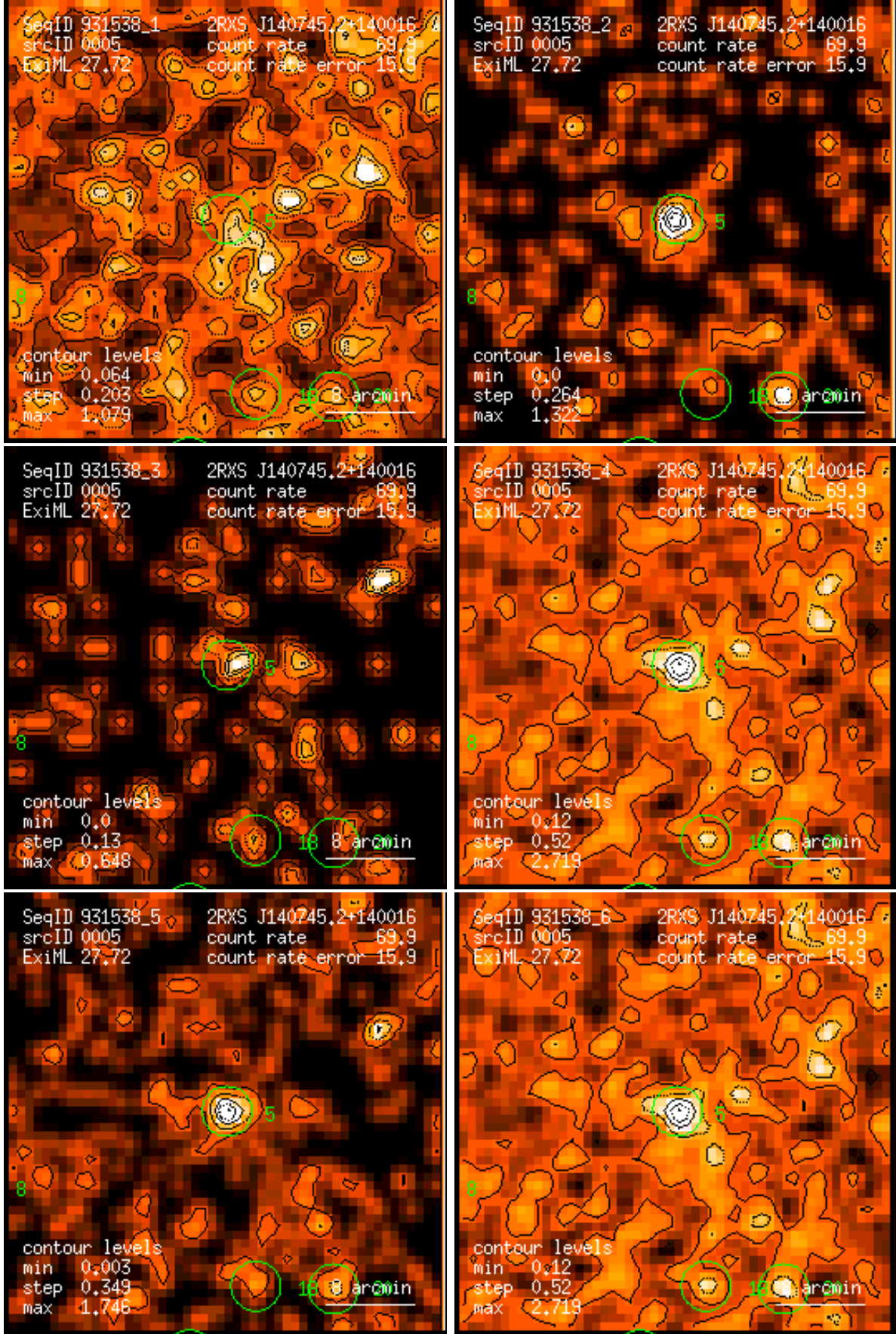
Figure 5: RASS 931538: detection 0005: band rate images, Gaussian filter: (1) PSPC channels 11 – 41, (2) 52 – 90, (3) 91 – 201, (4) 11 – 235, (5) 52 – 201, (6) 11 – 201. Broad band rates in counts/ks. Band rate contour levels in counts/ks/arcmin 2 .
