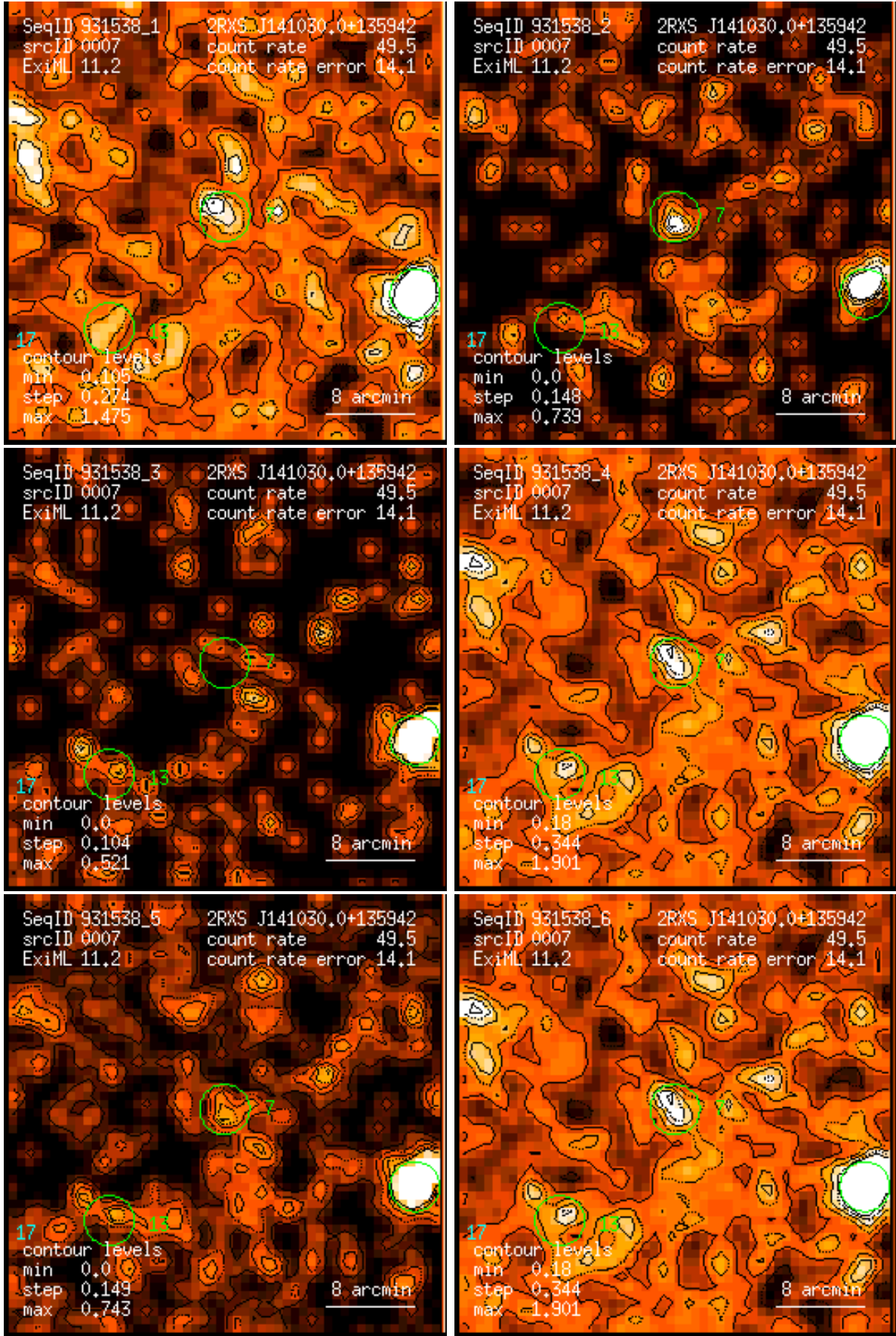
Figure 7: RASS 931538: detection 0007: band rate images, Gaussian filter: (1) PSPC channels 11 – 41, (2) 52 – 90, (3) 91 – 201, (4) 11 – 235, (5) 52 – 201, (6) 11 – 201. Broad band rates in counts/ks. Band rate contour levels in counts/ks/arcmin 2 .
