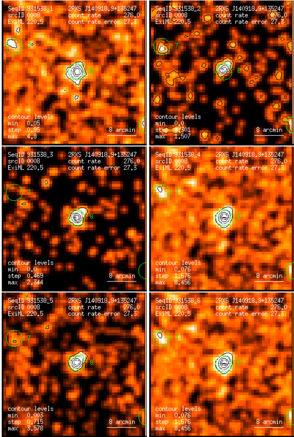
Figure 8: RASS 931538: detection 0008: band rate images, Gaussian filter: (1) PSPC channels 11 – 41, (2) 52 – 90, (3) 91 – 201, (4) 11 – 235, (5) 52 – 201, (6) 11 – 201. Broad band rates in counts/ks. Band rate contour levels in counts/ks/arcmin 2 .
