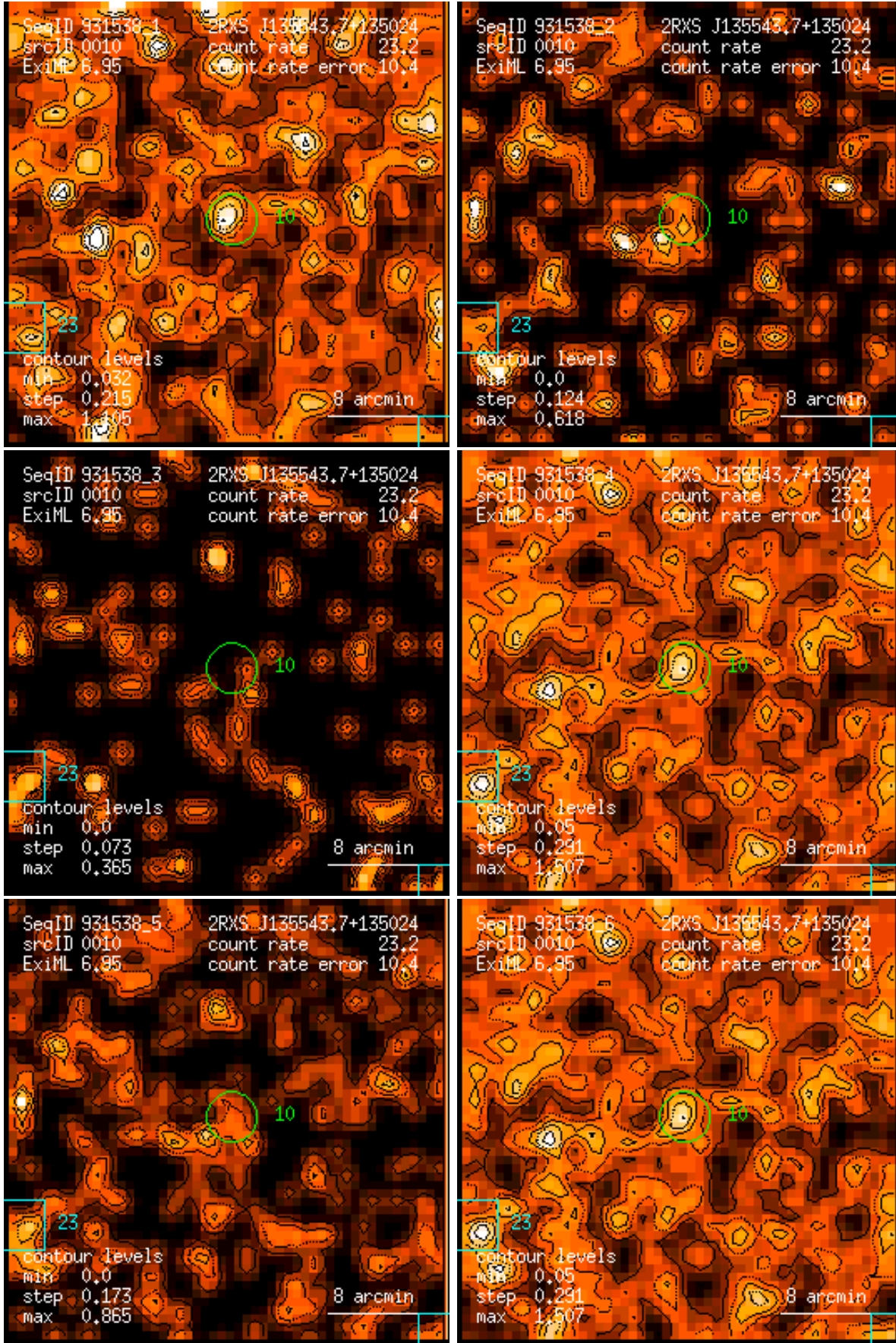
Figure 10: RASS 931538: detection 0010: band rate images, Gaussian filter: (1) PSPC channels 11 – 41, (2) 52 – 90, (3) 91 – 201, (4) 11 – 235, (5) 52 – 201, (6) 11 – 201. Broad band rates in counts/ks. Band rate contour levels in counts/ks/arcmin 2 .
