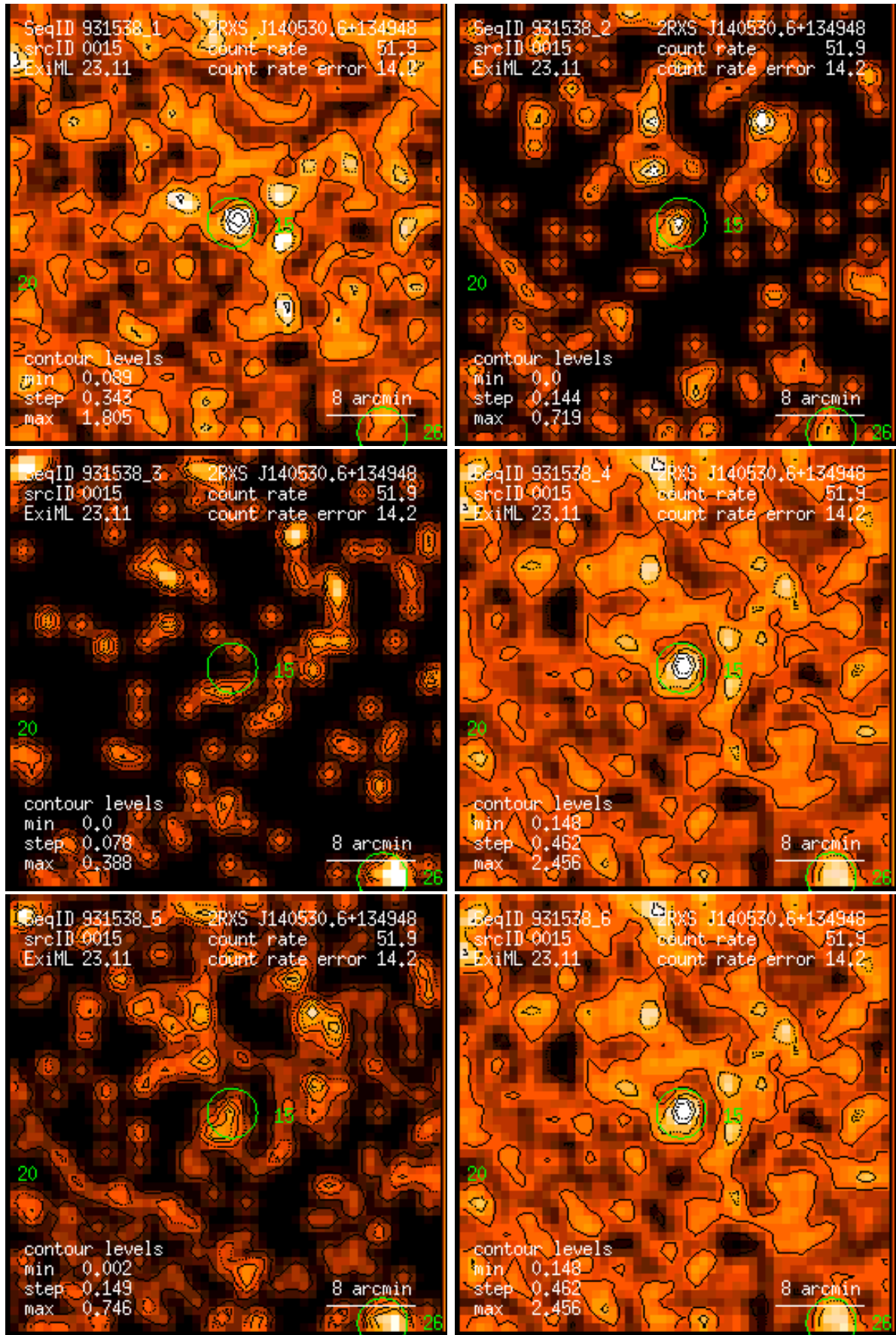
Figure 15: RASS 931538: detection 0015: band rate images, Gaussian filter: (1) PSPC channels 11 – 41, (2) 52 – 90, (3) 91 – 201, (4) 11 – 235, (5) 52 – 201, (6) 11 – 201. Broad band rates in counts/ks. Band rate contour levels in counts/ks/arcmin 2 .
