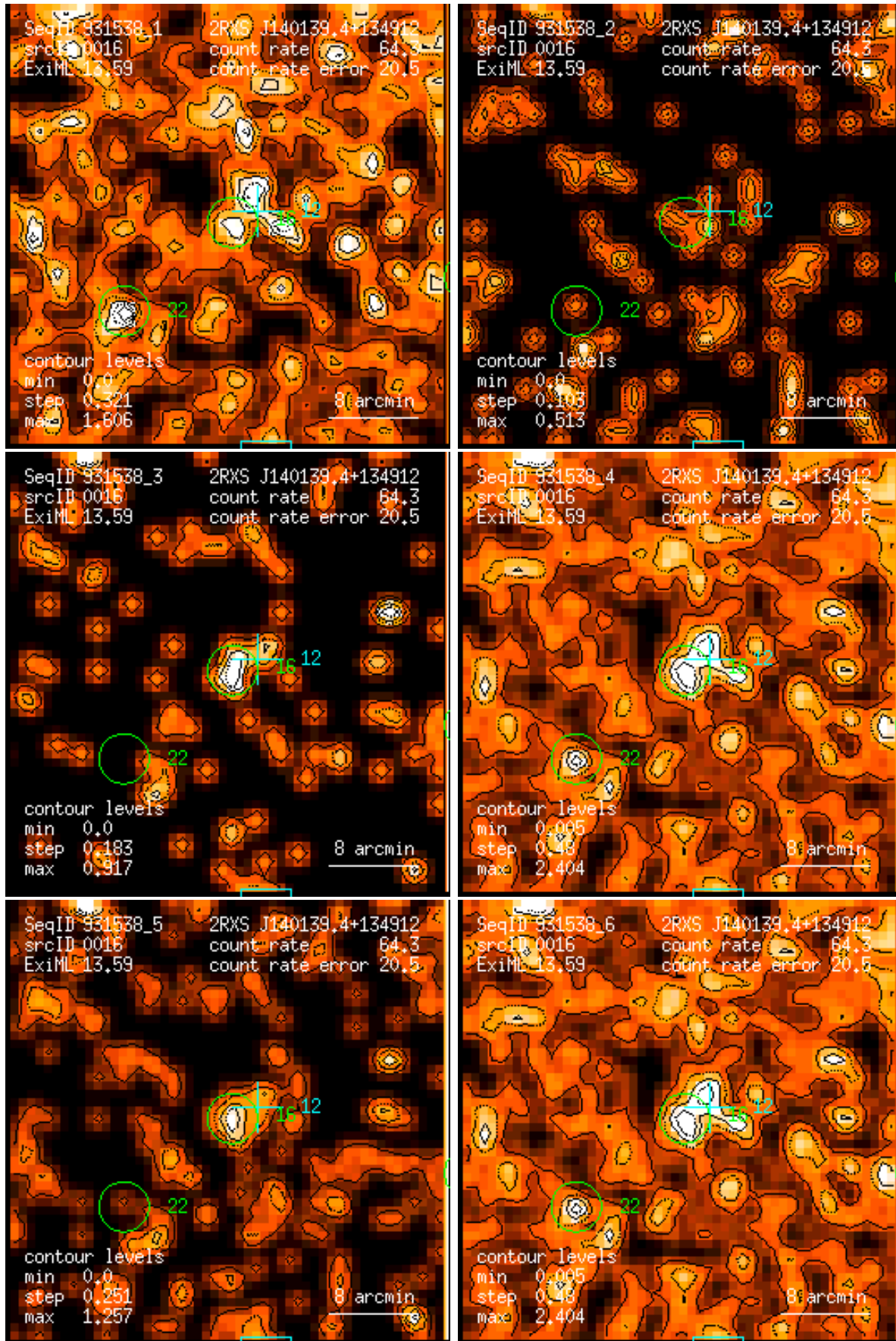
Figure 16: RASS 931538: detection 0016: band rate images, Gaussian filter: (1) PSPC channels 11 – 41, (2) 52 – 90, (3) 91 – 201, (4) 11 – 235, (5) 52 – 201, (6) 11 – 201. Broad band rates in counts/ks. Band rate contour levels in counts/ks/arcmin 2 .
