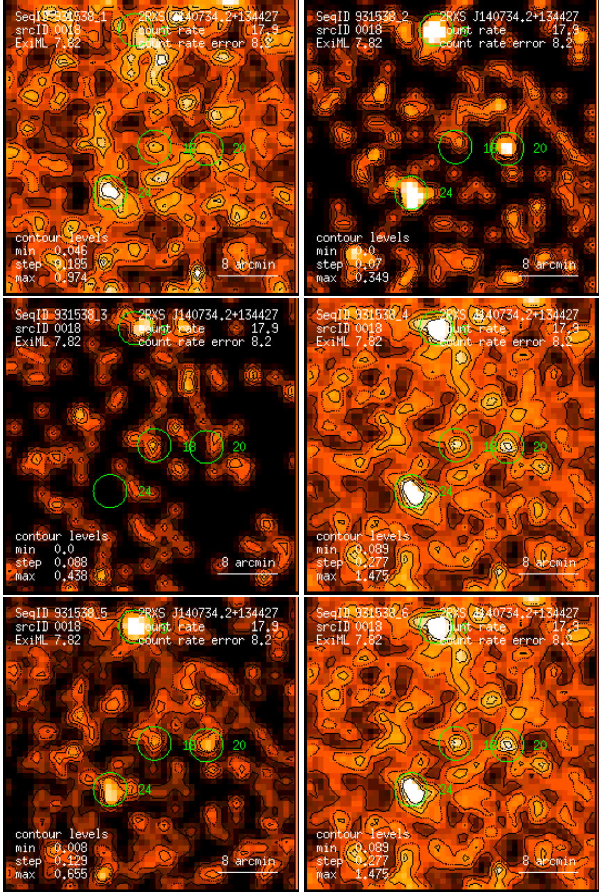
Figure 18: RASS 931538: detection 0018: band rate images, Gaussian filter: (1) PSPC channels 11 – 41, (2) 52 – 90, (3) 91 – 201, (4) 11 – 235, (5) 52 – 201, (6) 11 – 201. Broad band rates in counts/ks. Band rate contour levels in counts/ks/arcmin 2 .
