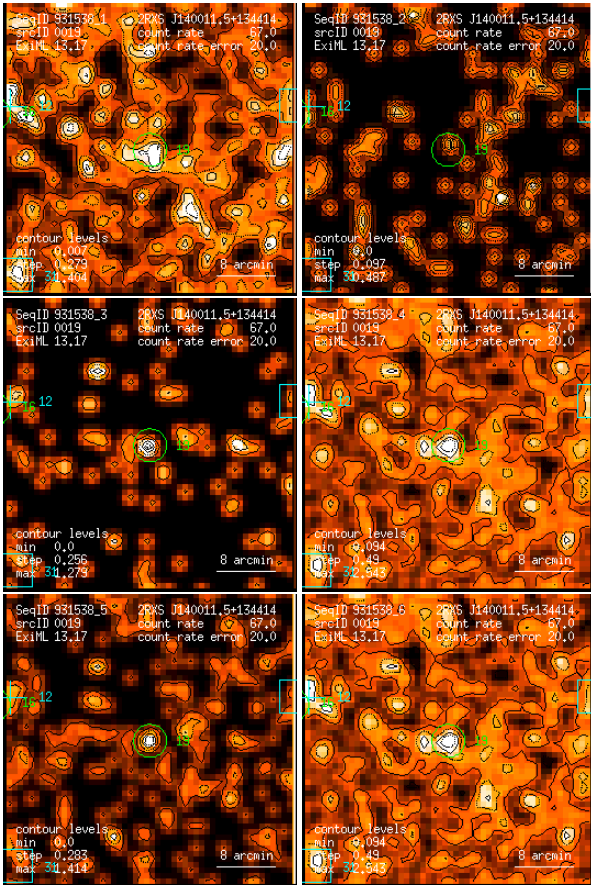
Figure 19: RASS 931538: detection 0019: band rate images, Gaussian filter: (1) PSPC channels 11 – 41, (2) 52 – 90, (3) 91 – 201, (4) 11 – 235, (5) 52 – 201, (6) 11 – 201. Broad band rates in counts/ks. Band rate contour levels in counts/ks/arcmin 2 .
