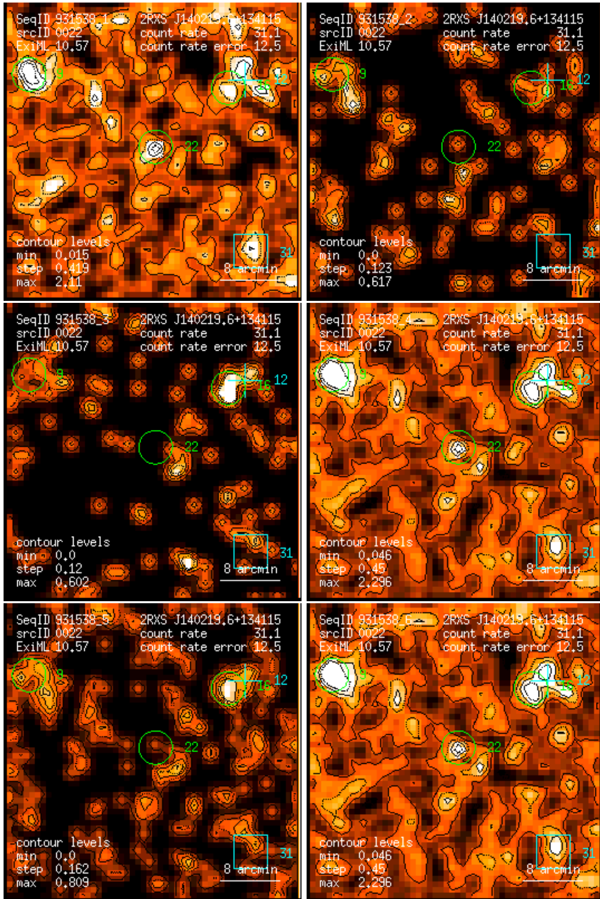
Figure 22: RASS 931538: detection 0022: band rate images, Gaussian filter: (1) PSPC channels 11 – 41, (2) 52 – 90, (3) 91 – 201, (4) 11 – 235, (5) 52 – 201, (6) 11 – 201. Broad band rates in counts/ks. Band rate contour levels in counts/ks/arcmin 2 .
