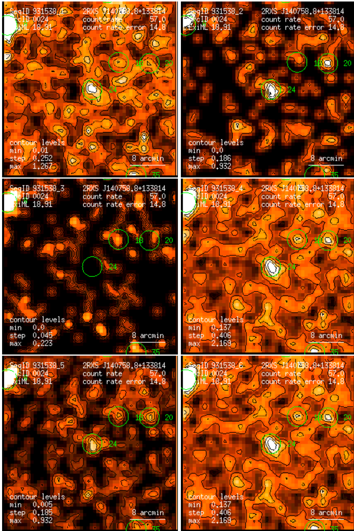
Figure 24: RASS 931538: detection 0024: band rate images, Gaussian filter: (1) PSPC channels 11 – 41, (2) 52 – 90, (3) 91 – 201, (4) 11 – 235, (5) 52 – 201, (6) 11 – 201. Broad band rates in counts/ks. Band rate contour levels in counts/ks/arcmin 2 .
