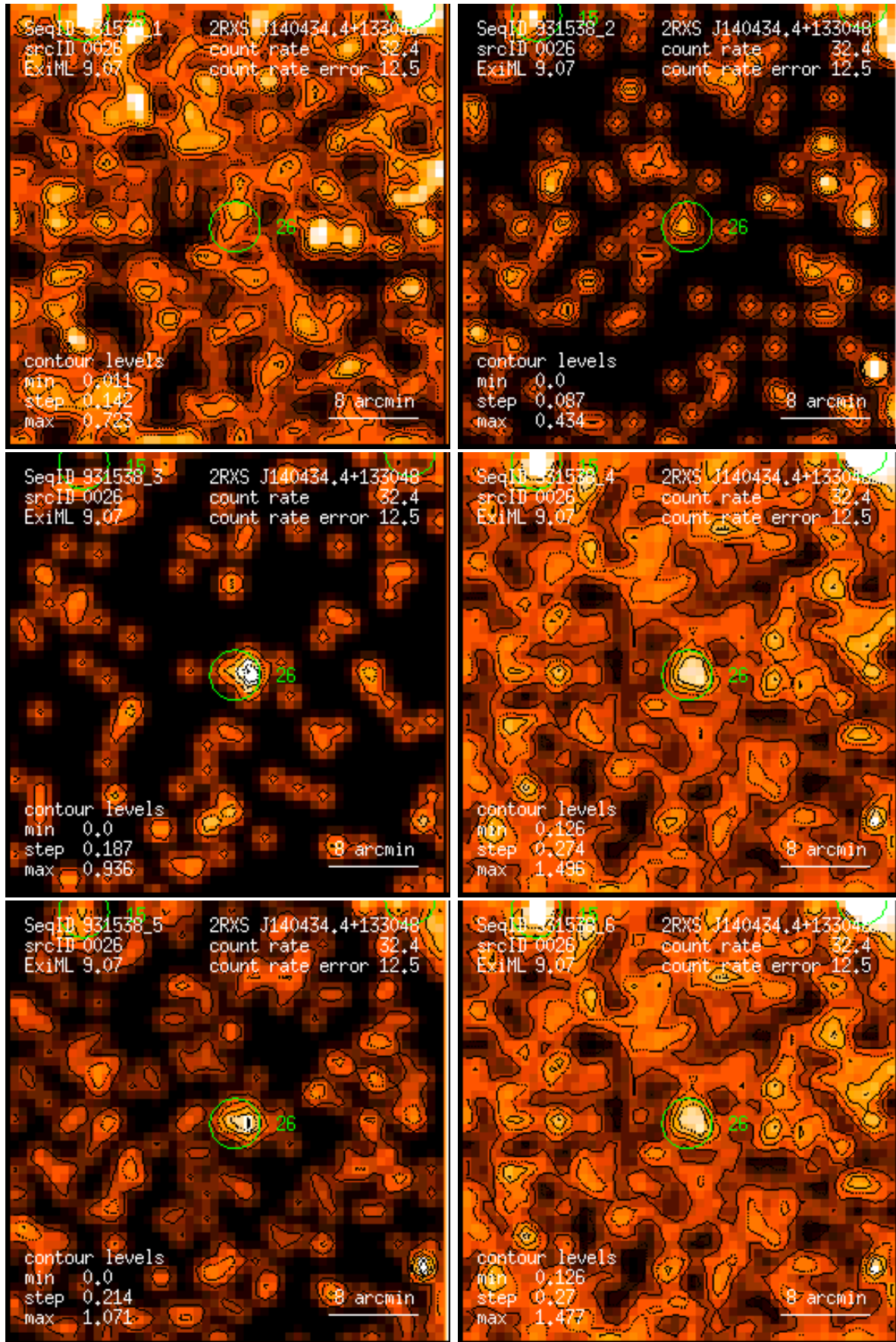
Figure 26: RASS 931538: detection 0026: band rate images, Gaussian filter: (1) PSPC channels 11 – 41, (2) 52 – 90, (3) 91 – 201, (4) 11 – 235, (5) 52 – 201, (6) 11 – 201. Broad band rates in counts/ks. Band rate contour levels in counts/ks/arcmin 2 .
