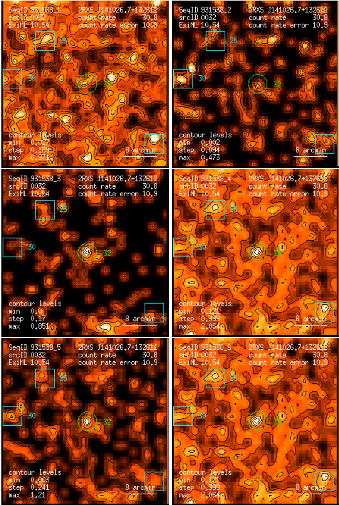
Figure 32: RASS 931538: detection 0032: band rate images, Gaussian filter: (1) PSPC channels 11 – 41, (2) 52 – 90, (3) 91 – 201, (4) 11 – 235, (5) 52 – 201, (6) 11 – 201. Broad band rates in counts/ks. Band rate contour levels in counts/ks/arcmin 2 .
