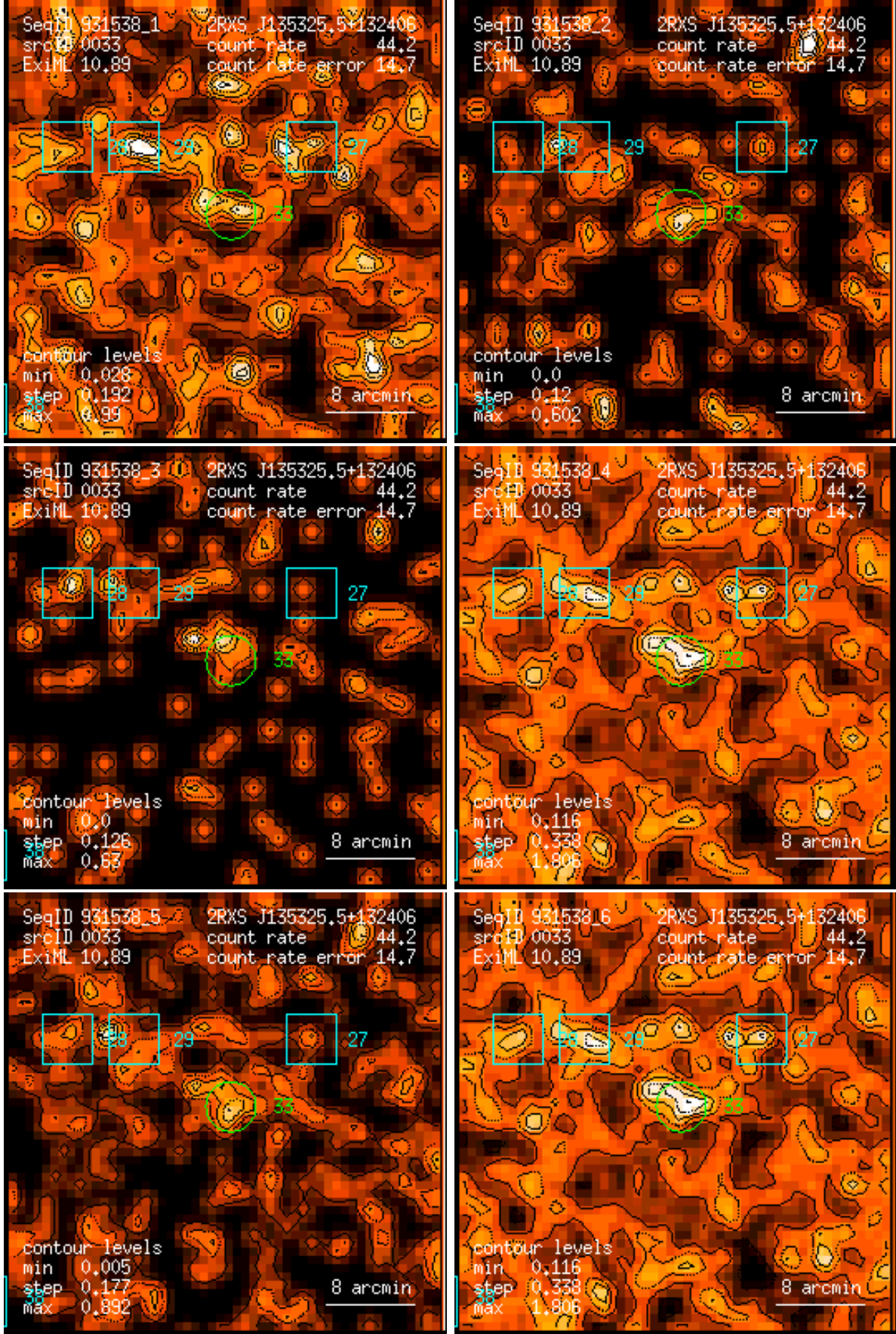
Figure 33: RASS 931538: detection 0033: band rate images, Gaussian filter: (1) PSPC channels 11 – 41, (2) 52 – 90, (3) 91 – 201, (4) 11 – 235, (5) 52 – 201, (6) 11 – 201. Broad band rates in counts/ks. Band rate contour levels in counts/ks/arcmin 2 .
