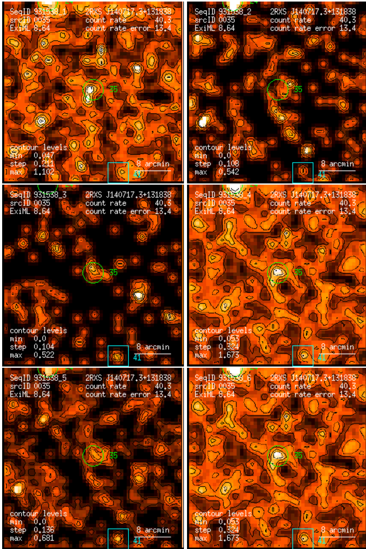
Figure 35: RASS 931538: detection 0035: band rate images, Gaussian filter: (1) PSPC channels 11 – 41, (2) 52 – 90, (3) 91 – 201, (4) 11 – 235, (5) 52 – 201, (6) 11 – 201. Broad band rates in counts/ks. Band rate contour levels in counts/ks/arcmin 2 .
