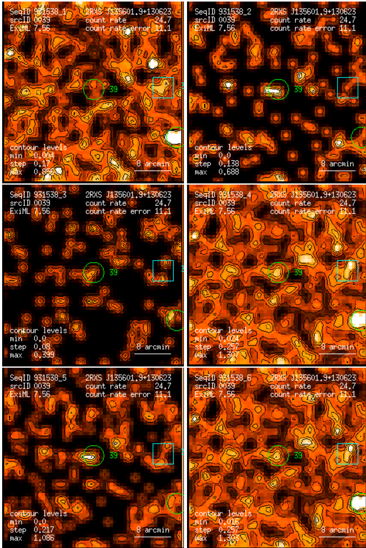
Figure 39: RASS 931538: detection 0039: band rate images, Gaussian filter: (1) PSPC channels 11 – 41, (2) 52 – 90, (3) 91 – 201, (4) 11 – 235, (5) 52 – 201, (6) 11 – 201. Broad band rates in counts/ks. Band rate contour levels in counts/ks/arcmin 2 .
