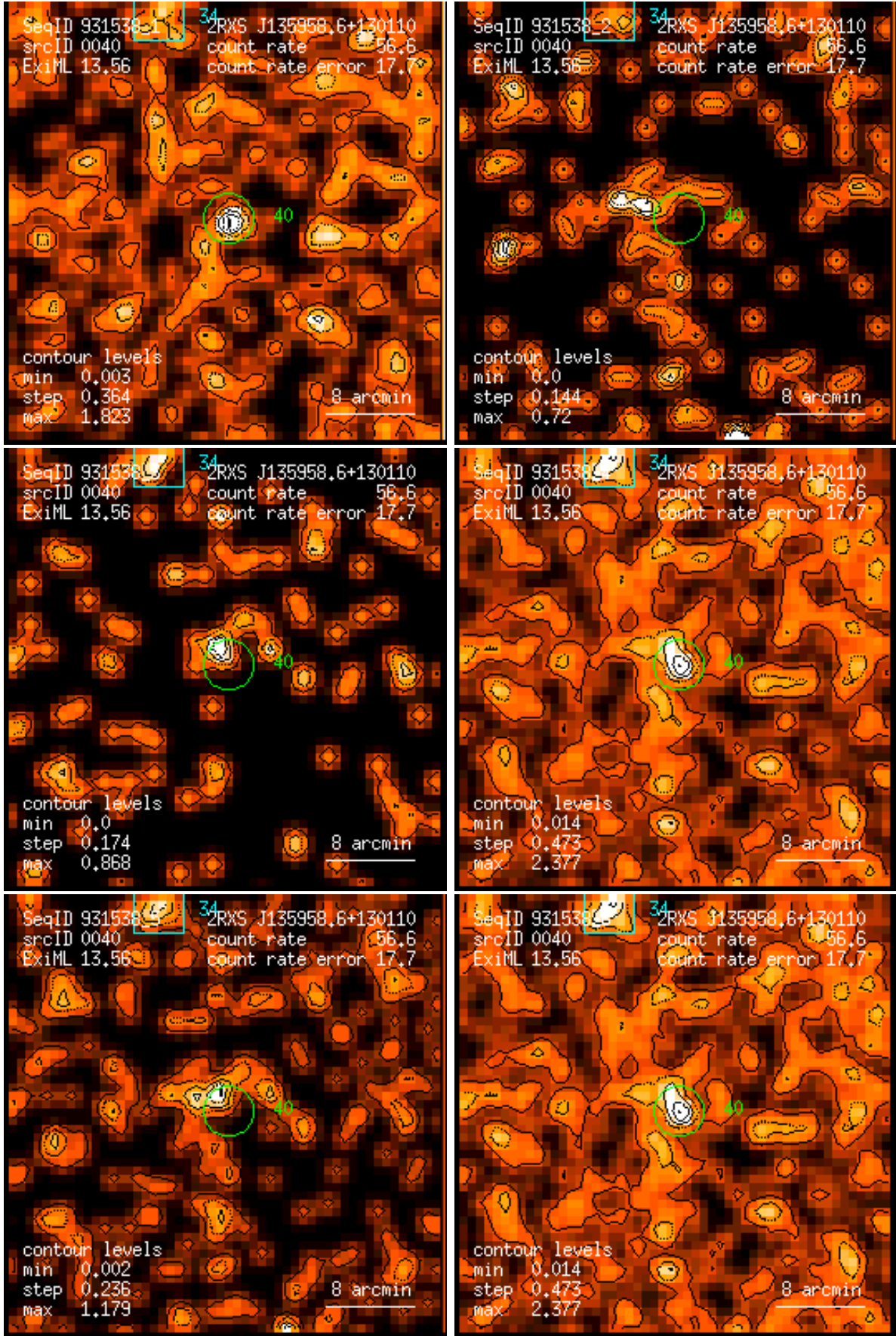
Figure 40: RASS 931538: detection 0040: band rate images, Gaussian filter: (1) PSPC channels 11 – 41, (2) 52 – 90, (3) 91 – 201, (4) 11 – 235, (5) 52 – 201, (6) 11 – 201. Broad band rates in counts/ks. Band rate contour levels in counts/ks/arcmin 2 .
