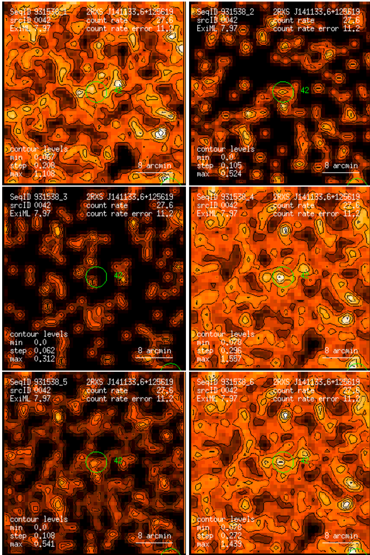
Figure 42: RASS 931538: detection 0042: band rate images, Gaussian filter: (1) PSPC channels 11 – 41, (2) 52 – 90, (3) 91 – 201, (4) 11 – 235, (5) 52 – 201, (6) 11 – 201. Broad band rates in counts/ks. Band rate contour levels in counts/ks/arcmin 2 .
