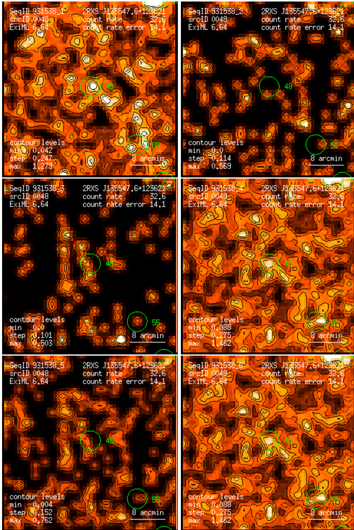
Figure 48: RASS 931538: detection 0048: band rate images, Gaussian filter: (1) PSPC channels 11 – 41, (2) 52 – 90, (3) 91 – 201, (4) 11 – 235, (5) 52 – 201, (6) 11 – 201. Broad band rates in counts/ks. Band rate contour levels in counts/ks/arcmin 2 .
