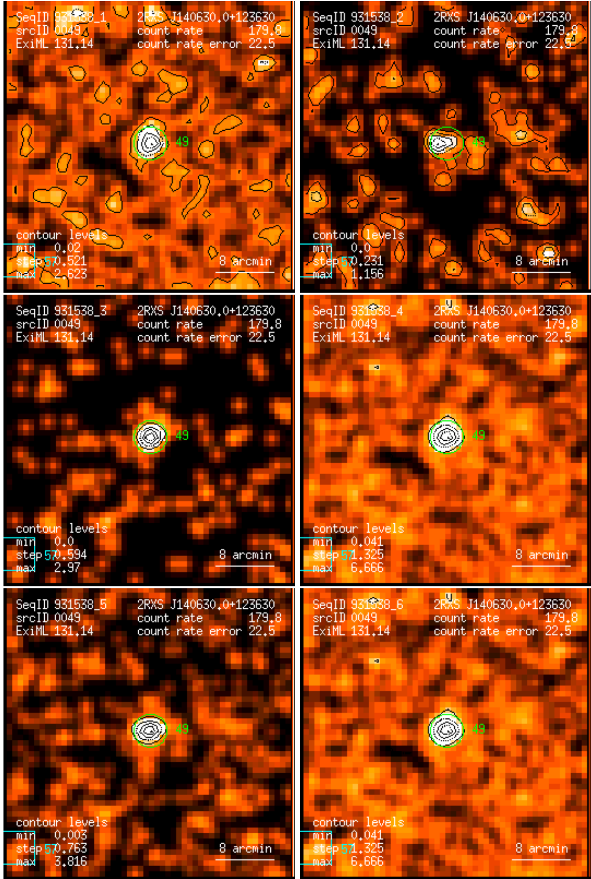
Figure 49: RASS 931538: detection 0049: band rate images, Gaussian filter: (1) PSPC channels 11 – 41, (2) 52 – 90, (3) 91 – 201, (4) 11 – 235, (5) 52 – 201, (6) 11 – 201. Broad band rates in counts/ks. Band rate contour levels in counts/ks/arcmin 2 .
