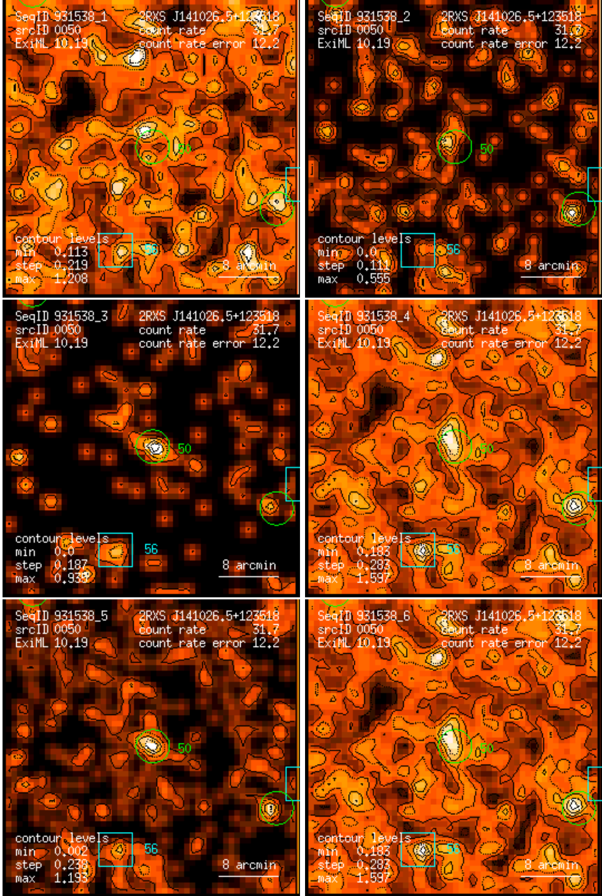
Figure 50: RASS 931538: detection 0050: band rate images, Gaussian filter: (1) PSPC channels 11 – 41, (2) 52 – 90, (3) 91 – 201, (4) 11 – 235, (5) 52 – 201, (6) 11 – 201. Broad band rates in counts/ks. Band rate contour levels in counts/ks/arcmin 2 .
