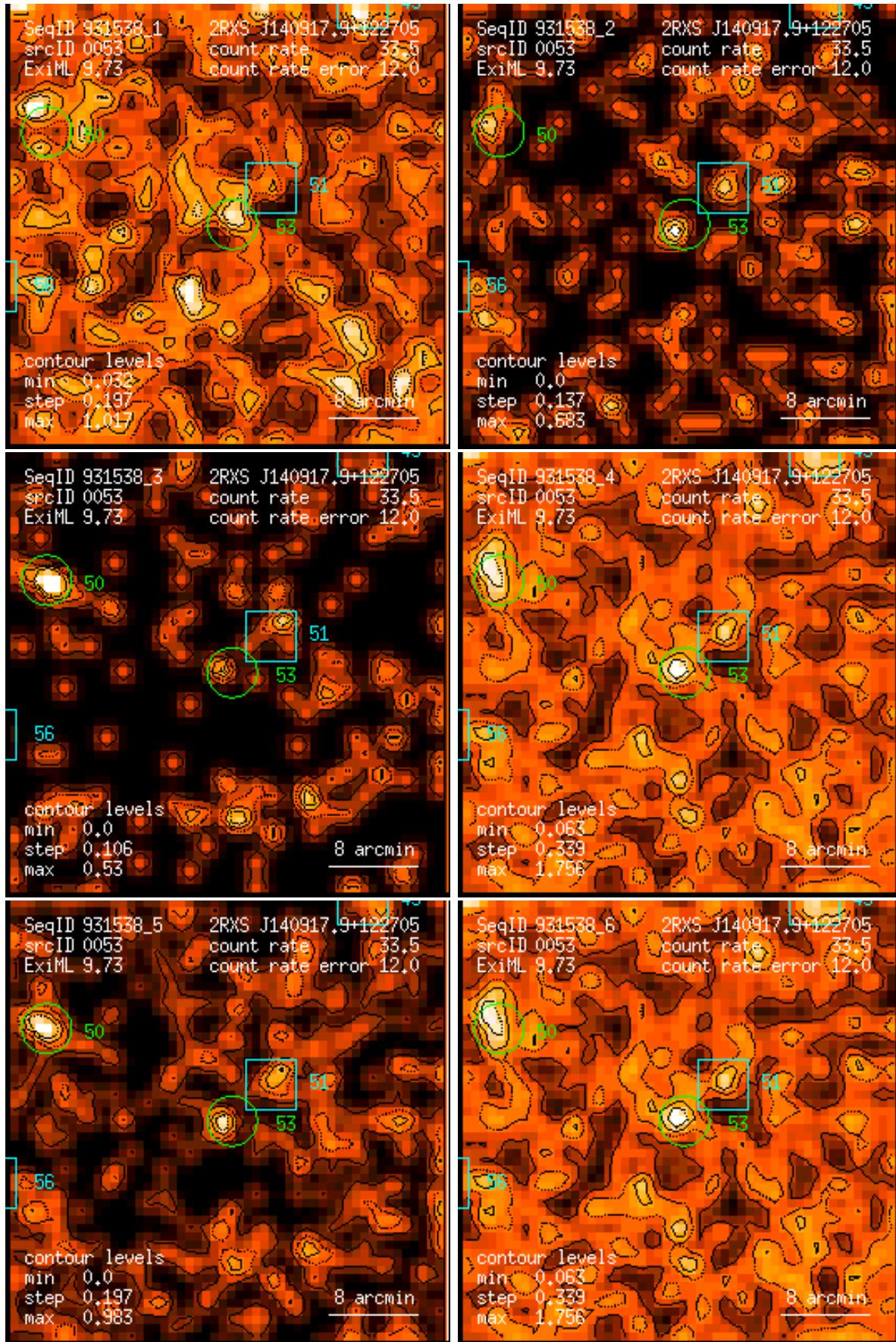
Figure 53: RASS 931538: detection 0053: band rate images, Gaussian filter: (1) PSPC channels 11 – 41, (2) 52 – 90, (3) 91 – 201, (4) 11 – 235, (5) 52 – 201, (6) 11 – 201. Broad band rates in counts/ks. Band rate contour levels in counts/ks/arcmin 2 .
