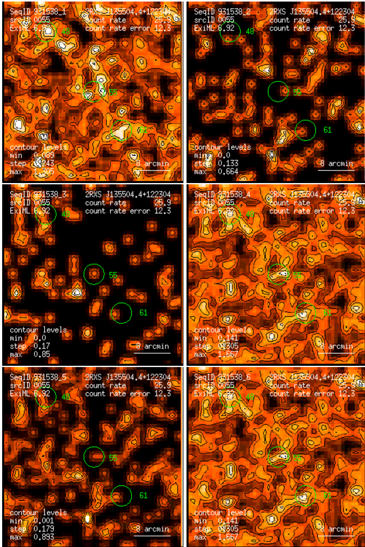
Figure 55: RASS 931538: detection 0055: band rate images, Gaussian filter: (1) PSPC channels 11 – 41, (2) 52 – 90, (3) 91 – 201, (4) 11 – 235, (5) 52 – 201, (6) 11 – 201. Broad band rates in counts/ks. Band rate contour levels in counts/ks/arcmin 2 .
