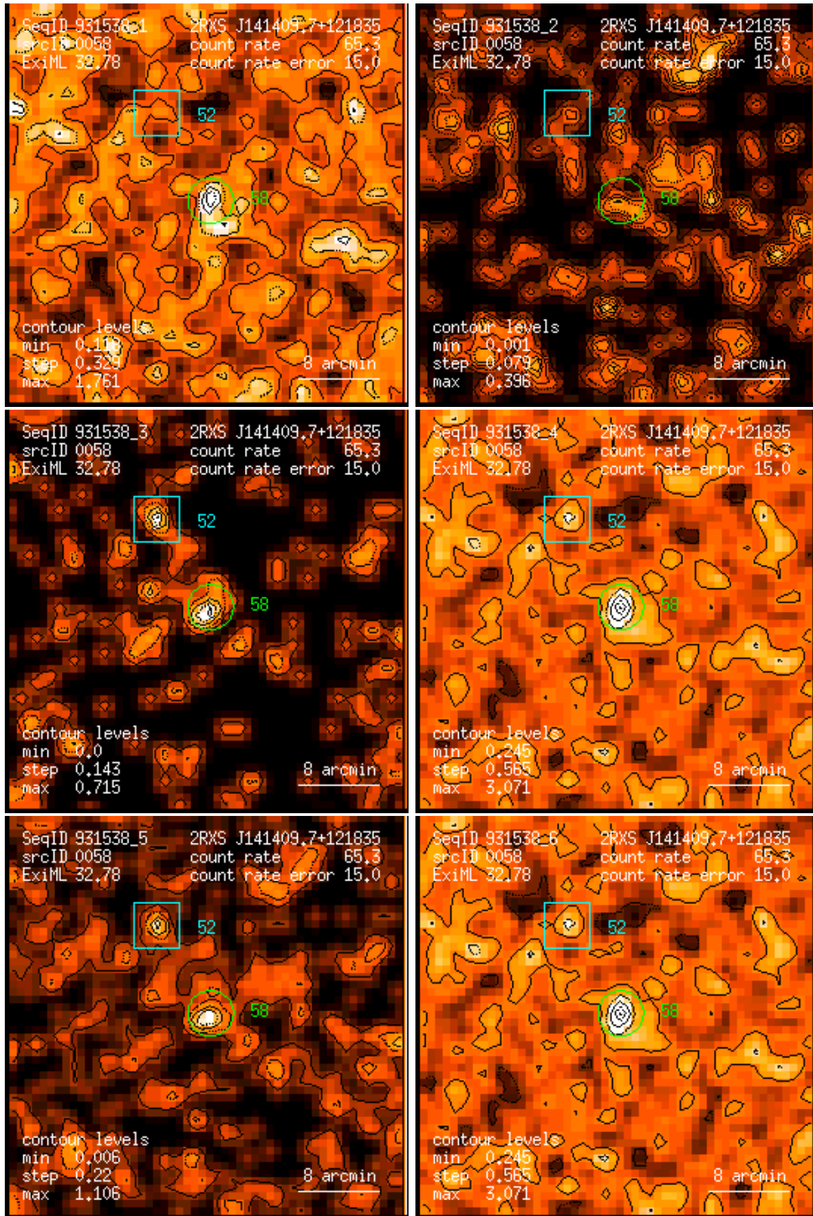
Figure 58: RASS 931538: detection 0058: band rate images, Gaussian filter: (1) PSPC channels 11 – 41, (2) 52 – 90, (3) 91 – 201, (4) 11 – 235, (5) 52 – 201, (6) 11 – 201. Broad band rates in counts/ks. Band rate contour levels in counts/ks/arcmin 2 .
