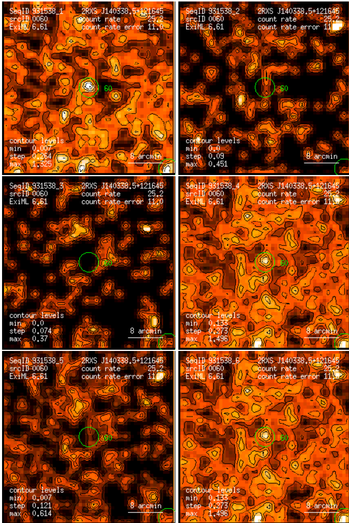
Figure 60: RASS 931538: detection 0060: band rate images, Gaussian filter: (1) PSPC channels 11 – 41, (2) 52 – 90, (3) 91 – 201, (4) 11 – 235, (5) 52 – 201, (6) 11 – 201. Broad band rates in counts/ks. Band rate contour levels in counts/ks/arcmin 2 .
