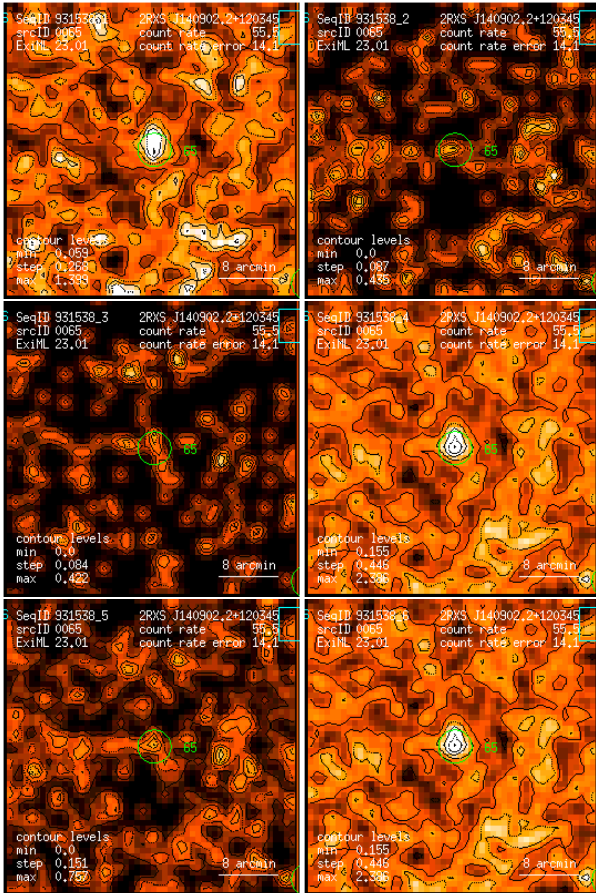
Figure 65: RASS 931538: detection 0065: band rate images, Gaussian filter: (1) PSPC channels 11 – 41, (2) 52 – 90, (3) 91 – 201, (4) 11 – 235, (5) 52 – 201, (6) 11 – 201. Broad band rates in counts/ks. Band rate contour levels in counts/ks/arcmin 2 .
