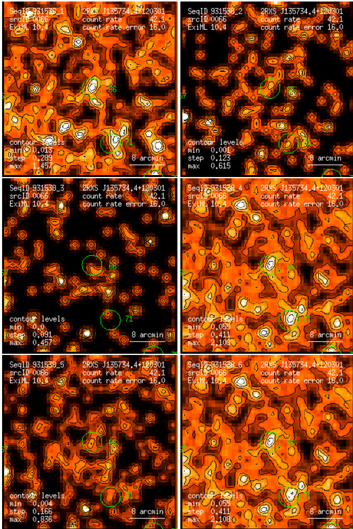
Figure 66: RASS 931538: detection 0066: band rate images, Gaussian filter: (1) PSPC channels 11 – 41, (2) 52 – 90, (3) 91 – 201, (4) 11 – 235, (5) 52 – 201, (6) 11 – 201. Broad band rates in counts/ks. Band rate contour levels in counts/ks/arcmin 2 .
