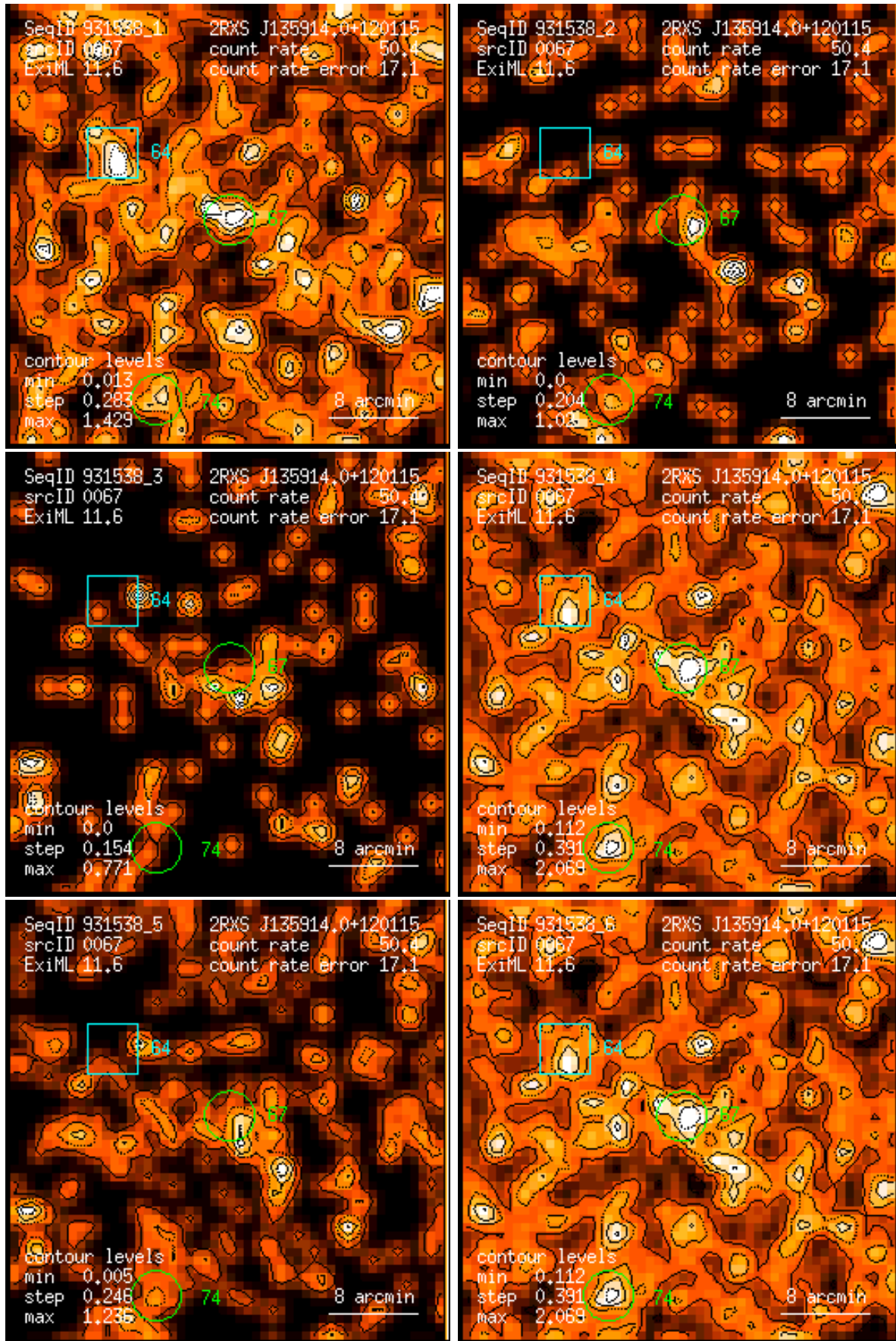
Figure 67: RASS 931538: detection 0067: band rate images, Gaussian filter: (1) PSPC channels 11 – 41, (2) 52 – 90, (3) 91 – 201, (4) 11 – 235, (5) 52 – 201, (6) 11 – 201. Broad band rates in counts/ks. Band rate contour levels in counts/ks/arcmin 2 .
