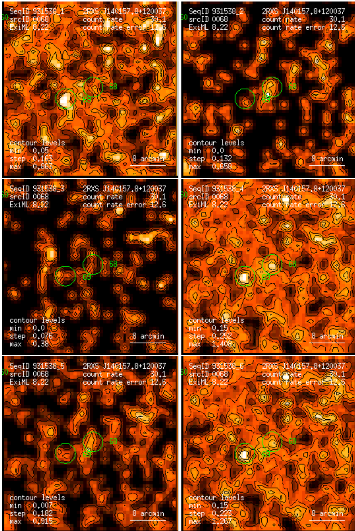
Figure 68: RASS 931538: detection 0068: band rate images, Gaussian filter: (1) PSPC channels 11 – 41, (2) 52 – 90, (3) 91 – 201, (4) 11 – 235, (5) 52 – 201, (6) 11 – 201. Broad band rates in counts/ks. Band rate contour levels in counts/ks/arcmin 2 .
