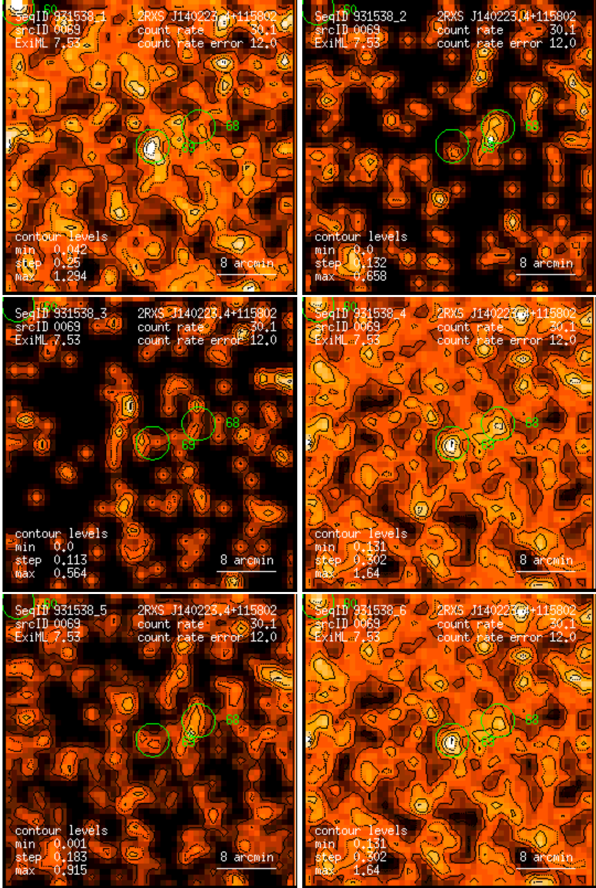
Figure 69: RASS 931538: detection 0069: band rate images, Gaussian filter: (1) PSPC channels 11 – 41, (2) 52 – 90, (3) 91 – 201, (4) 11 – 235, (5) 52 – 201, (6) 11 – 201. Broad band rates in counts/ks. Band rate contour levels in counts/ks/arcmin 2 .
