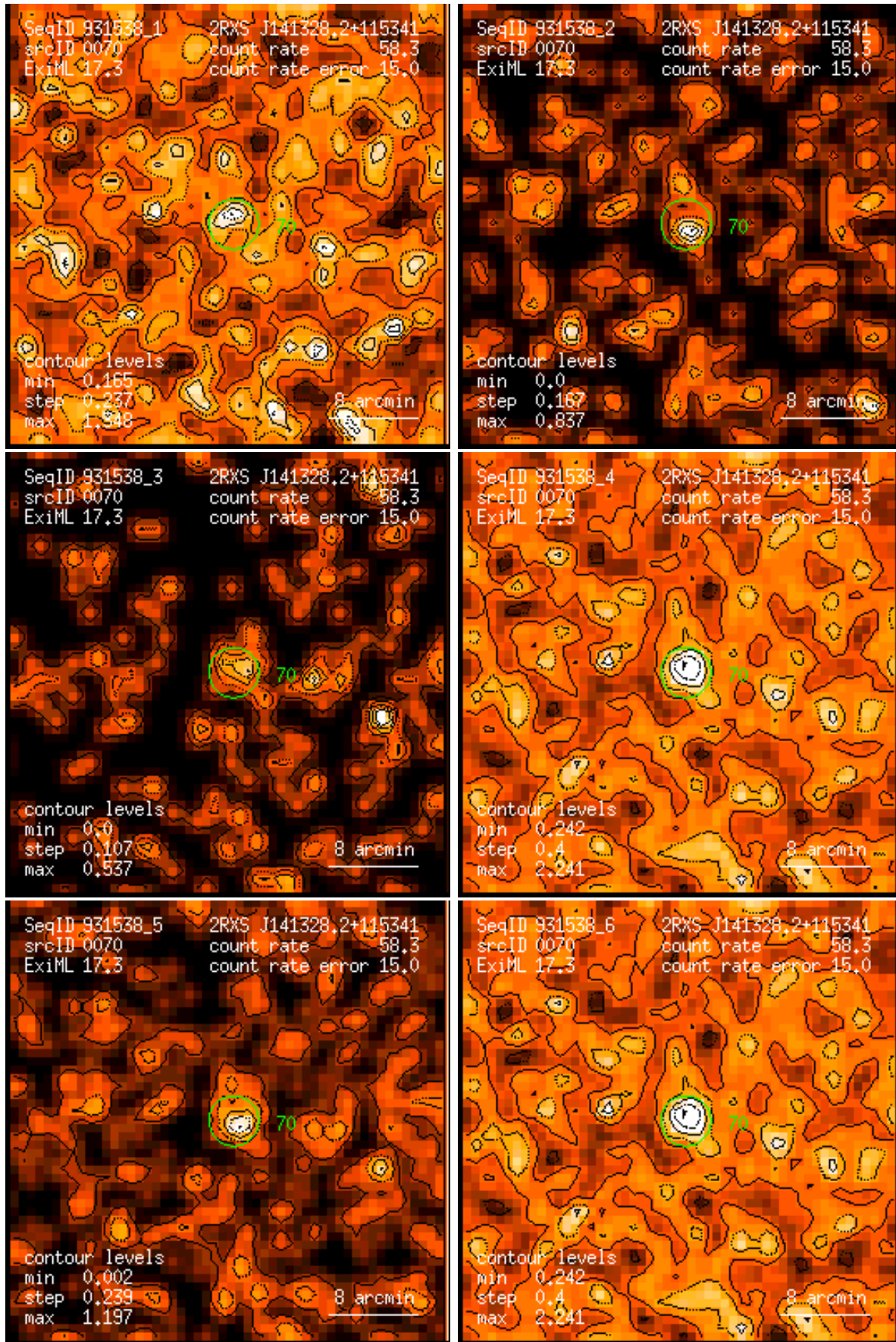
Figure 70: RASS 931538: detection 0070: band rate images, Gaussian filter: (1) PSPC channels 11 – 41, (2) 52 – 90, (3) 91 – 201, (4) 11 – 235, (5) 52 – 201, (6) 11 – 201. Broad band rates in counts/ks. Band rate contour levels in counts/ks/arcmin 2 .
