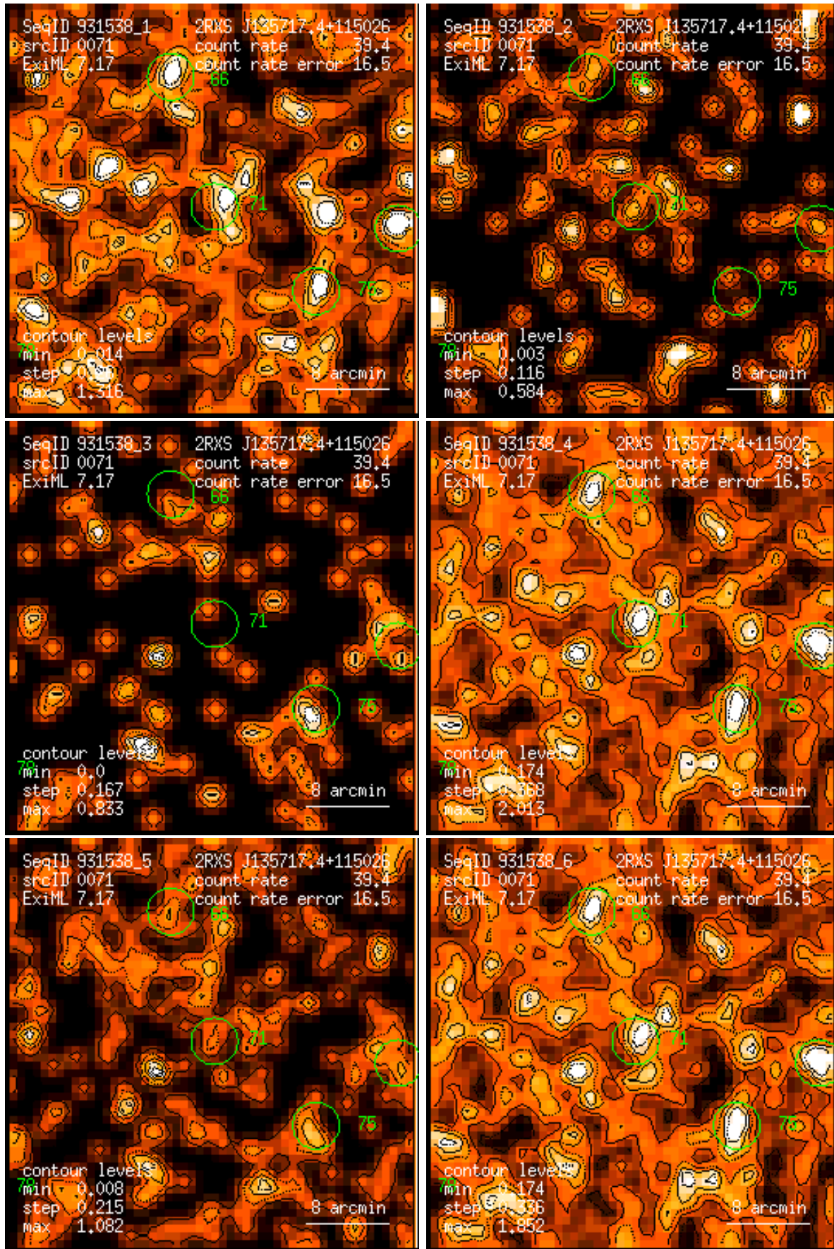
Figure 71: RASS 931538: detection 0071: band rate images, Gaussian filter: (1) PSPC channels 11 – 41, (2) 52 – 90, (3) 91 – 201, (4) 11 – 235, (5) 52 – 201, (6) 11 – 201. Broad band rates in counts/ks. Band rate contour levels in counts/ks/arcmin 2 .
