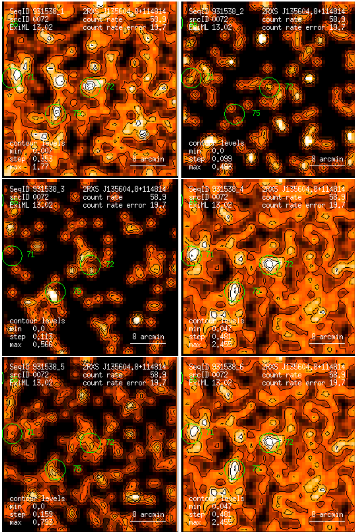
Figure 72: RASS 931538: detection 0072: band rate images, Gaussian filter: (1) PSPC channels 11 – 41, (2) 52 – 90, (3) 91 – 201, (4) 11 – 235, (5) 52 – 201, (6) 11 – 201. Broad band rates in counts/ks. Band rate contour levels in counts/ks/arcmin 2 .
