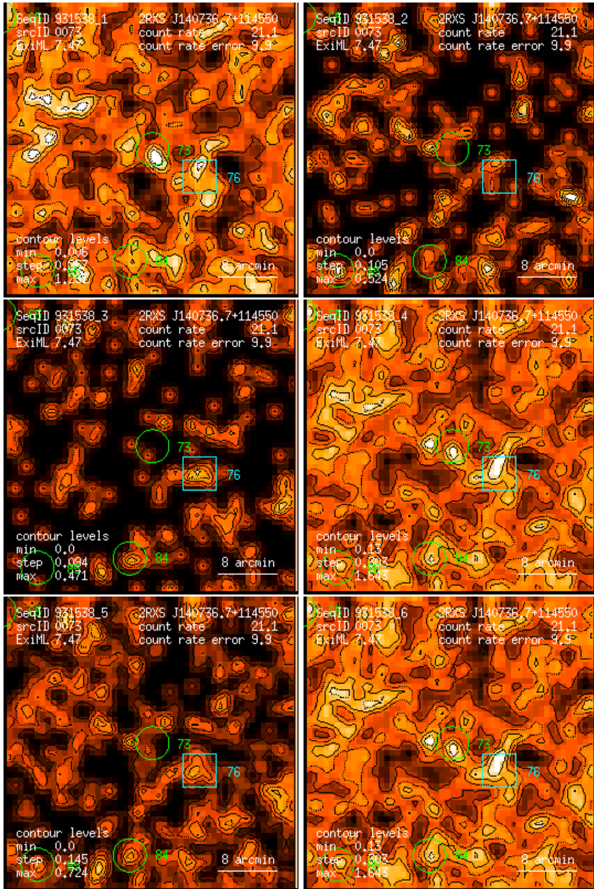
Figure 73: RASS 931538: detection 0073: band rate images, Gaussian filter: (1) PSPC channels 11 – 41, (2) 52 – 90, (3) 91 – 201, (4) 11 – 235, (5) 52 – 201, (6) 11 – 201. Broad band rates in counts/ks. Band rate contour levels in counts/ks/arcmin 2 .
