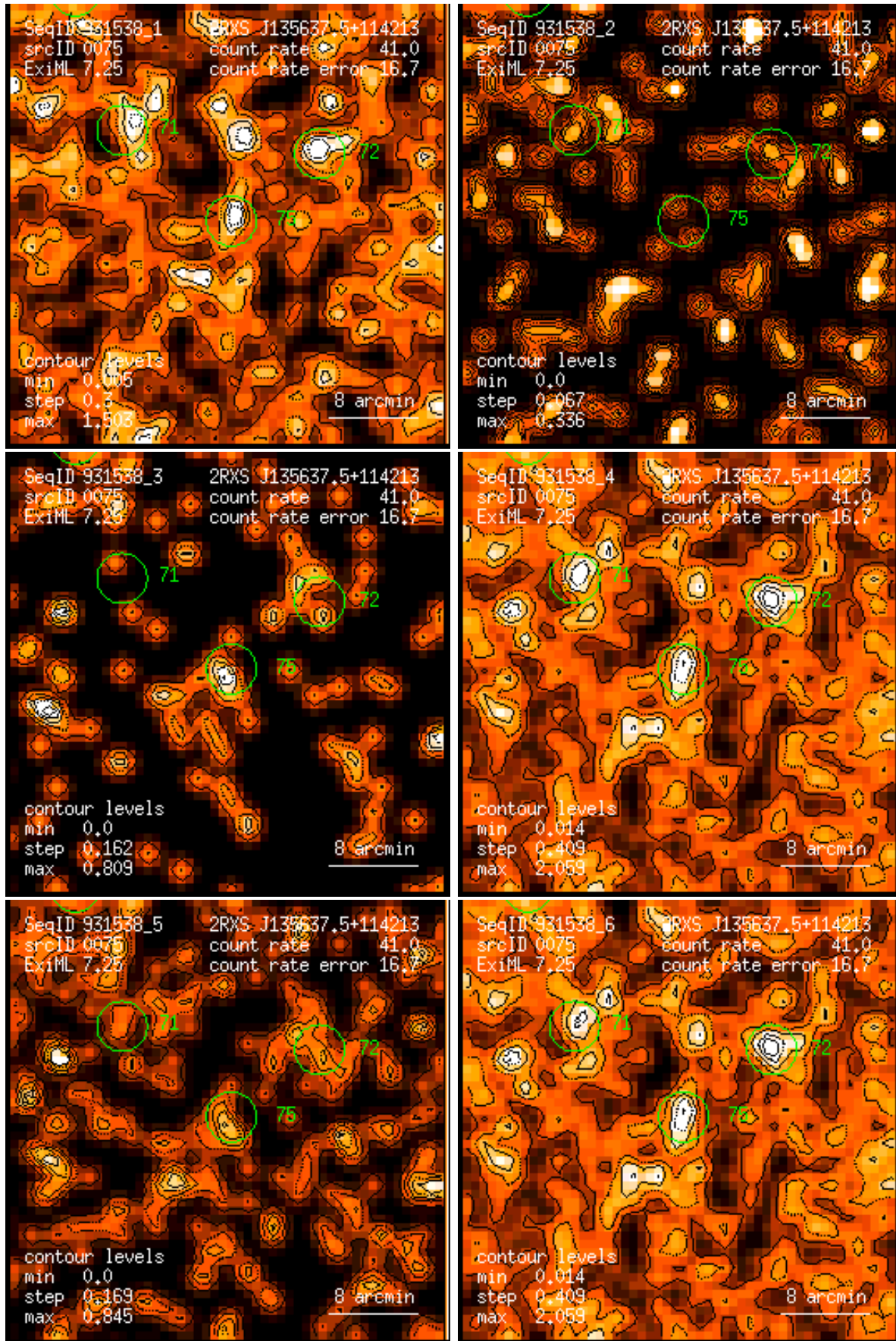
Figure 75: RASS 931538: detection 0075: band rate images, Gaussian filter: (1) PSPC channels 11 – 41, (2) 52 – 90, (3) 91 – 201, (4) 11 – 235, (5) 52 – 201, (6) 11 – 201. Broad band rates in counts/ks. Band rate contour levels in counts/ks/arcmin 2 .
