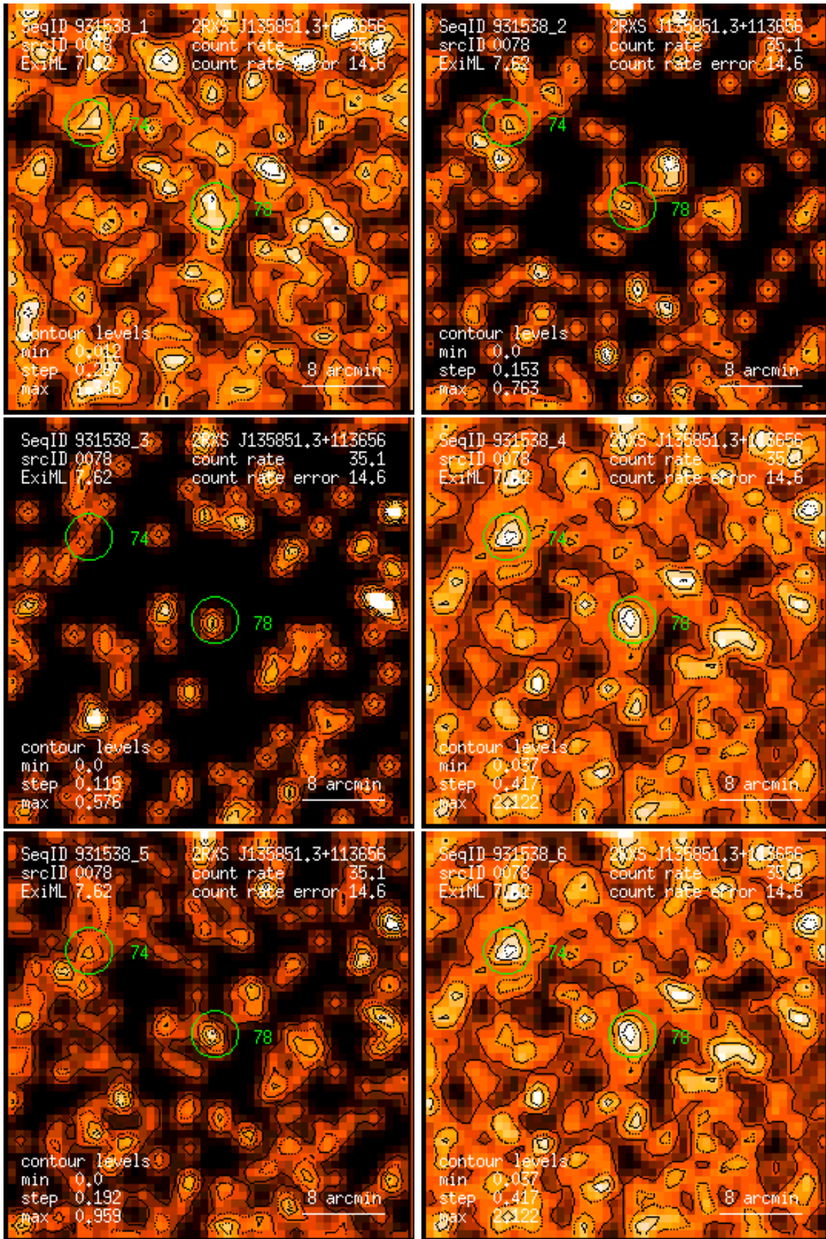
Figure 78: RASS 931538: detection 0078: band rate images, Gaussian filter: (1) PSPC channels 11 – 41, (2) 52 – 90, (3) 91 – 201, (4) 11 – 235, (5) 52 – 201, (6) 11 – 201. Broad band rates in counts/ks. Band rate contour levels in counts/ks/arcmin 2 .
