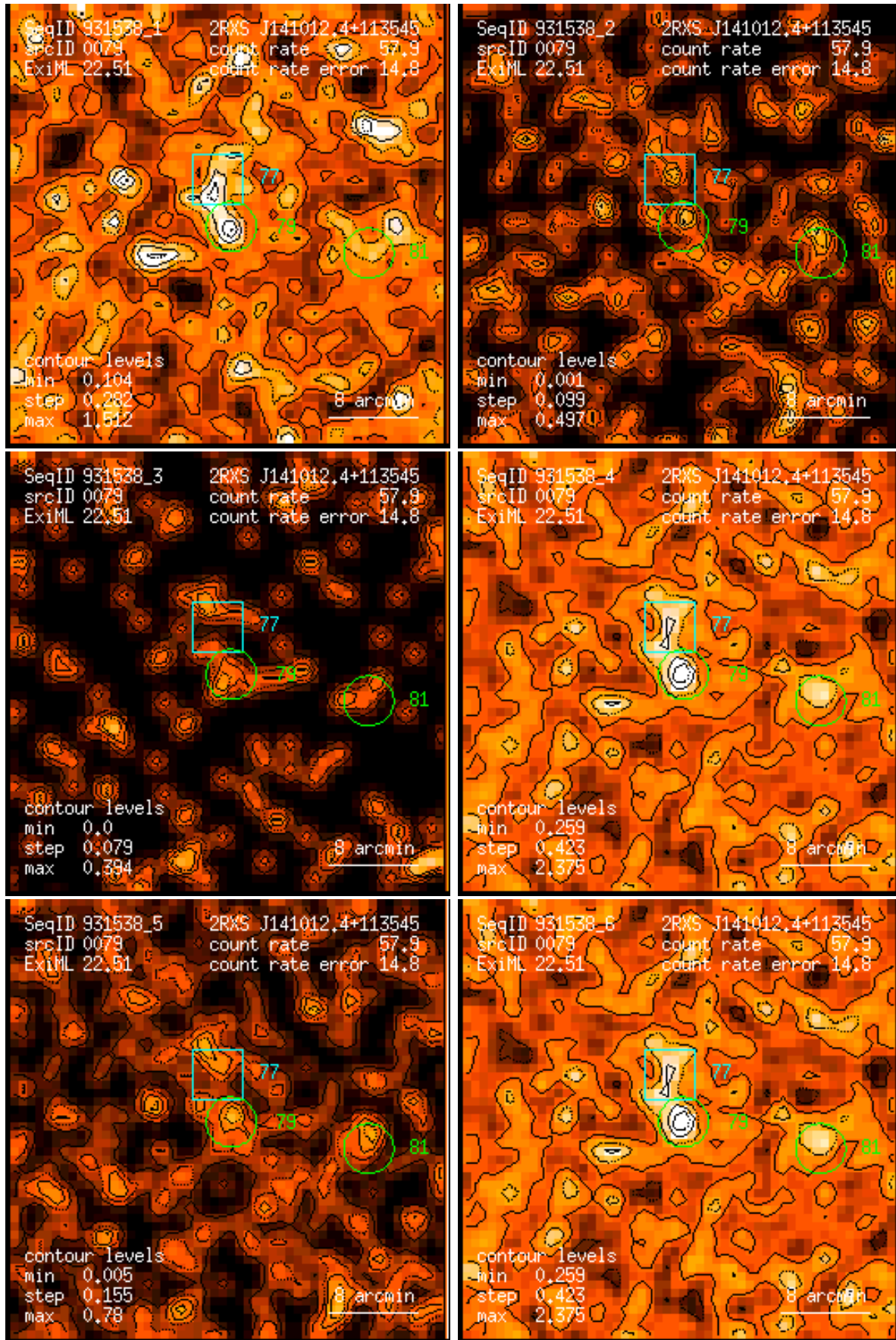
Figure 79: RASS 931538: detection 0079: band rate images, Gaussian filter: (1) PSPC channels 11 – 41, (2) 52 – 90, (3) 91 – 201, (4) 11 – 235, (5) 52 – 201, (6) 11 – 201. Broad band rates in counts/ks. Band rate contour levels in counts/ks/arcmin 2 .
