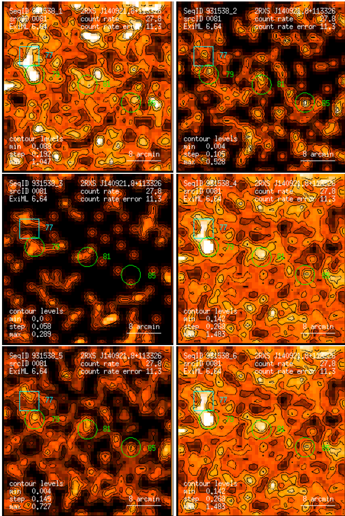
Figure 81: RASS 931538: detection 0081: band rate images, Gaussian filter: (1) PSPC channels 11 – 41, (2) 52 – 90, (3) 91 – 201, (4) 11 – 235, (5) 52 – 201, (6) 11 – 201. Broad band rates in counts/ks. Band rate contour levels in counts/ks/arcmin 2 .
