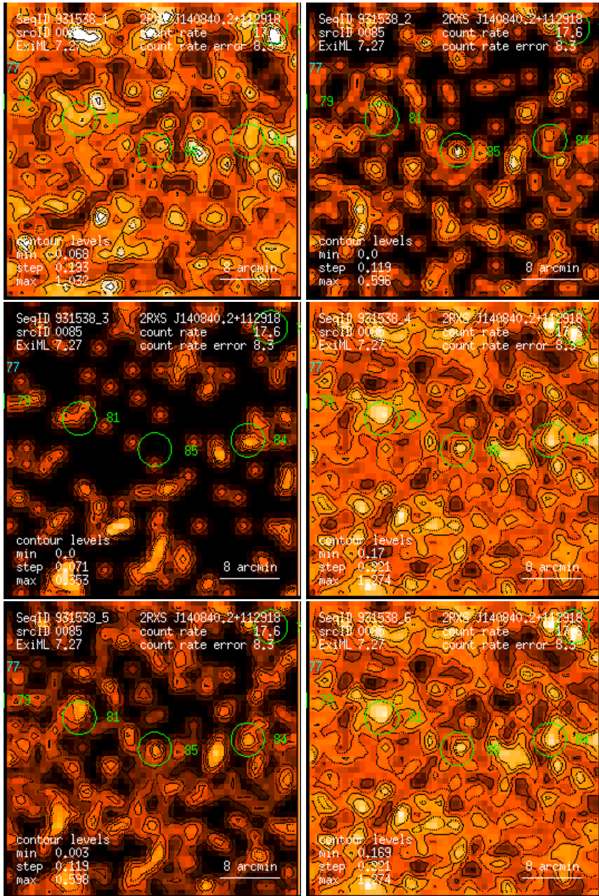
Figure 85: RASS 931538: detection 0085: band rate images, Gaussian filter: (1) PSPC channels 11 – 41, (2) 52 – 90, (3) 91 – 201, (4) 11 – 235, (5) 52 – 201, (6) 11 – 201. Broad band rates in counts/ks. Band rate contour levels in counts/ks/arcmin 2 .
