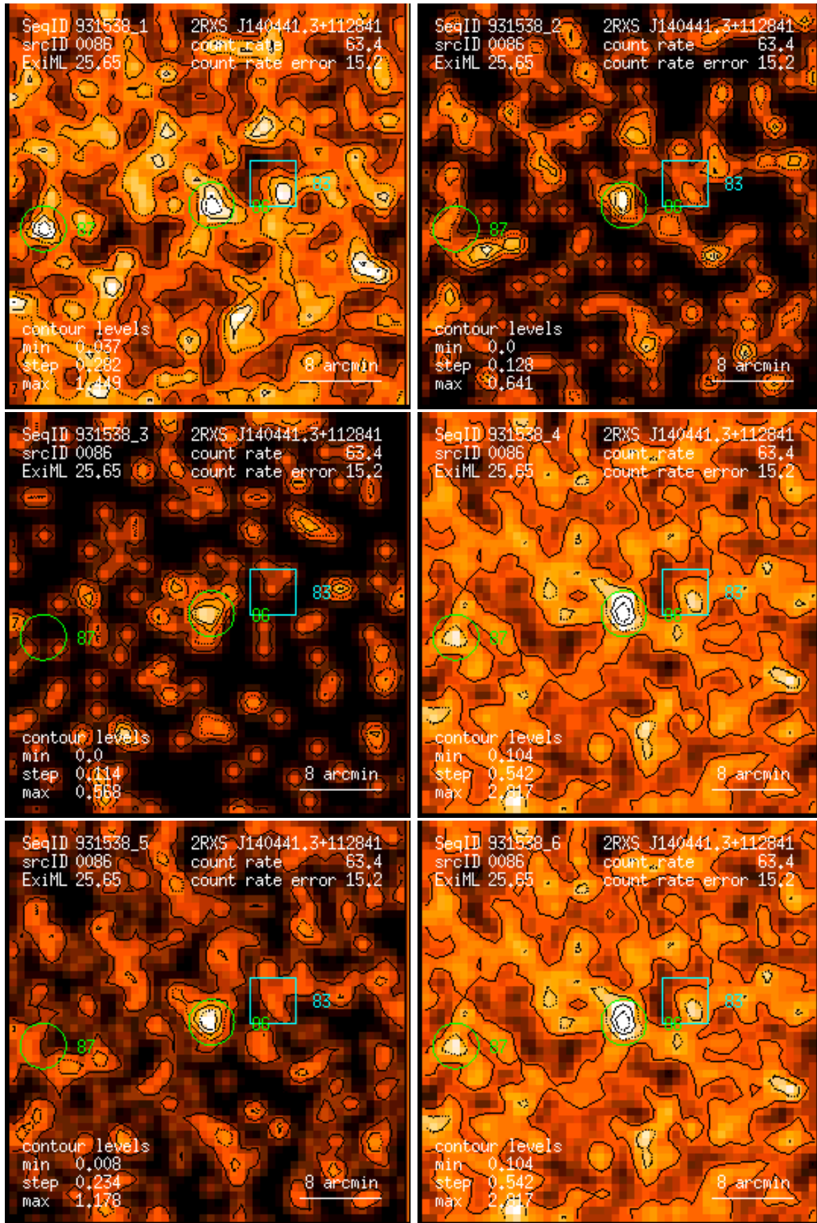
Figure 86: RASS 931538: detection 0086: band rate images, Gaussian filter: (1) PSPC channels 11 – 41, (2) 52 – 90, (3) 91 – 201, (4) 11 – 235, (5) 52 – 201, (6) 11 – 201. Broad band rates in counts/ks. Band rate contour levels in counts/ks/arcmin 2 .
