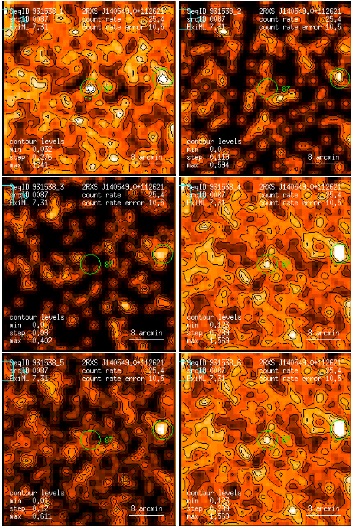
Figure 87: RASS 931538: detection 0087: band rate images, Gaussian filter: (1) PSPC channels 11 – 41, (2) 52 – 90, (3) 91 – 201, (4) 11 – 235, (5) 52 – 201, (6) 11 – 201. Broad band rates in counts/ks. Band rate contour levels in counts/ks/arcmin 2 .
