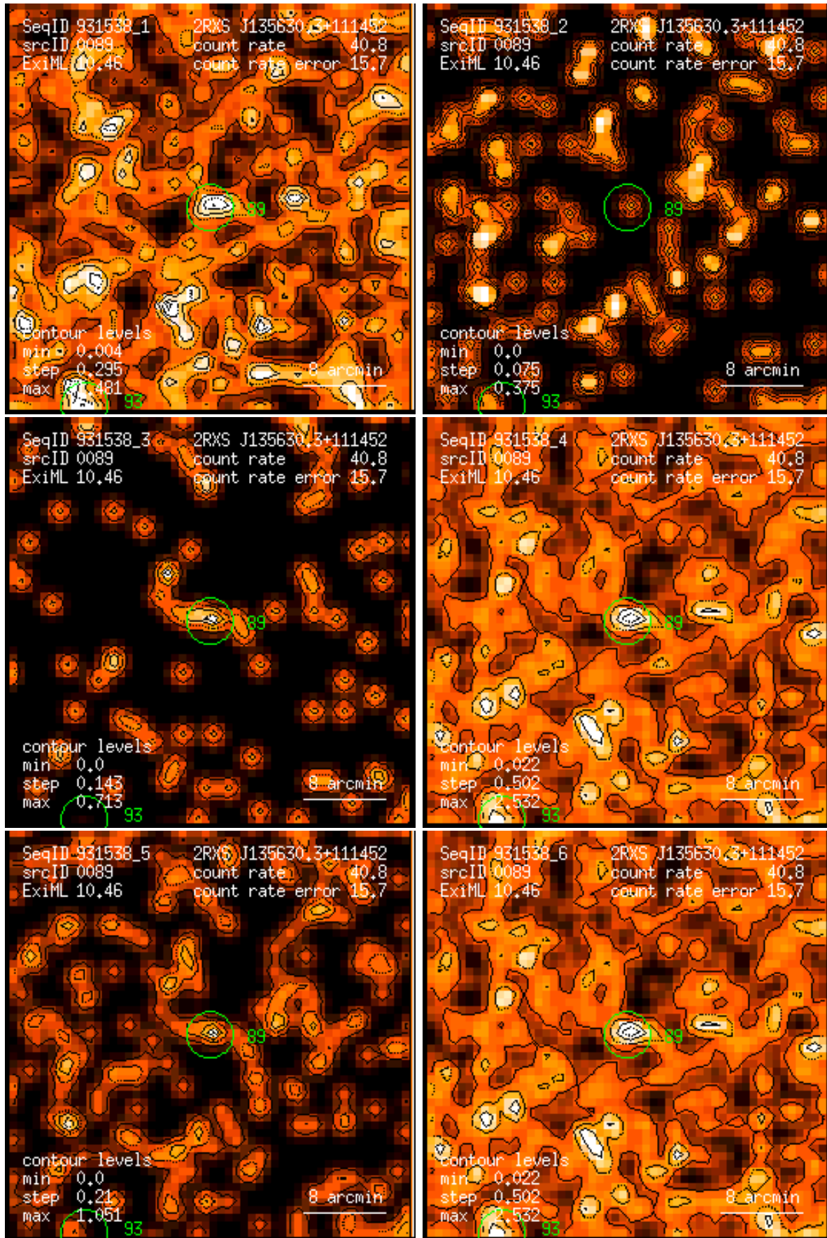
Figure 89: RASS 931538: detection 0089: band rate images, Gaussian filter: (1) PSPC channels 11 – 41, (2) 52 – 90, (3) 91 – 201, (4) 11 – 235, (5) 52 – 201, (6) 11 – 201. Broad band rates in counts/ks. Band rate contour levels in counts/ks/arcmin 2 .
