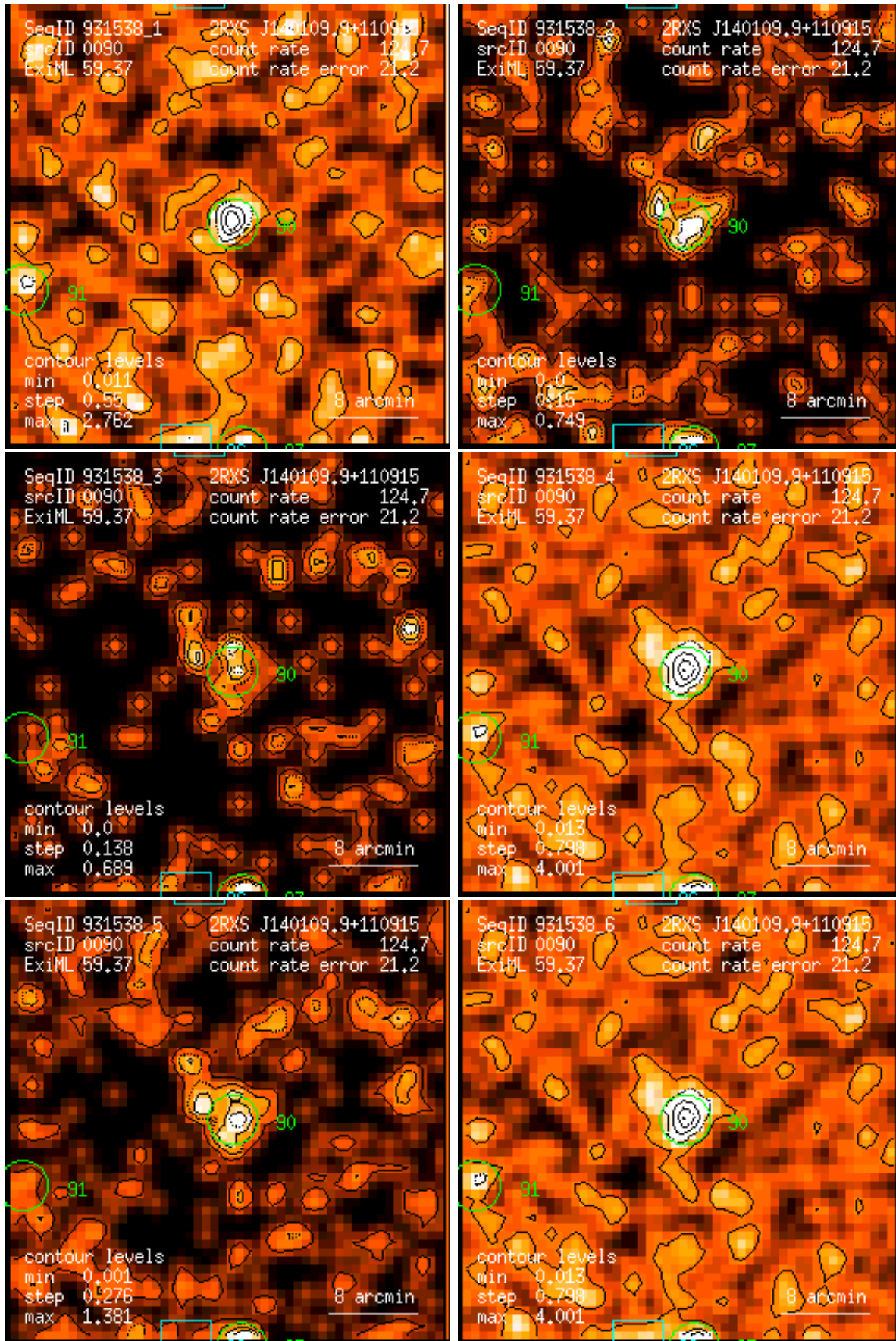
Figure 90: RASS 931538: detection 0090: band rate images, Gaussian filter: (1) PSPC channels 11 – 41, (2) 52 – 90, (3) 91 – 201, (4) 11 – 235, (5) 52 – 201, (6) 11 – 201. Broad band rates in counts/ks. Band rate contour levels in counts/ks/arcmin 2 .
