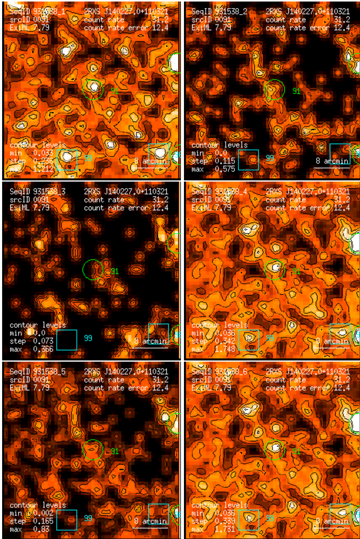
Figure 91: RASS 931538: detection 0091: band rate images, Gaussian filter: (1) PSPC channels 11 – 41, (2) 52 – 90, (3) 91 – 201, (4) 11 – 235, (5) 52 – 201, (6) 11 – 201. Broad band rates in counts/ks. Band rate contour levels in counts/ks/arcmin 2 .
