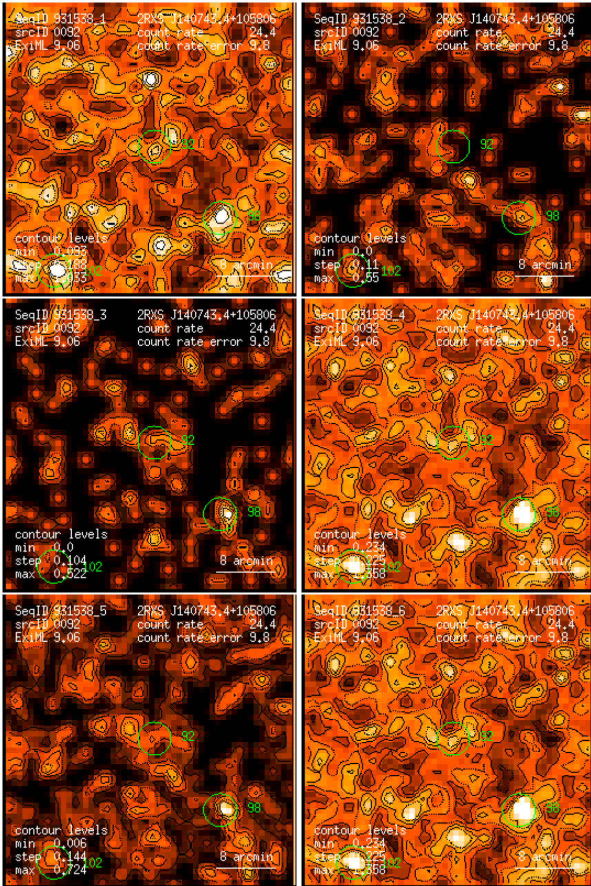
Figure 92: RASS 931538: detection 0092: band rate images, Gaussian filter: (1) PSPC channels 11 – 41, (2) 52 – 90, (3) 91 – 201, (4) 11 – 235, (5) 52 – 201, (6) 11 – 201. Broad band rates in counts/ks. Band rate contour levels in counts/ks/arcmin 2 .
