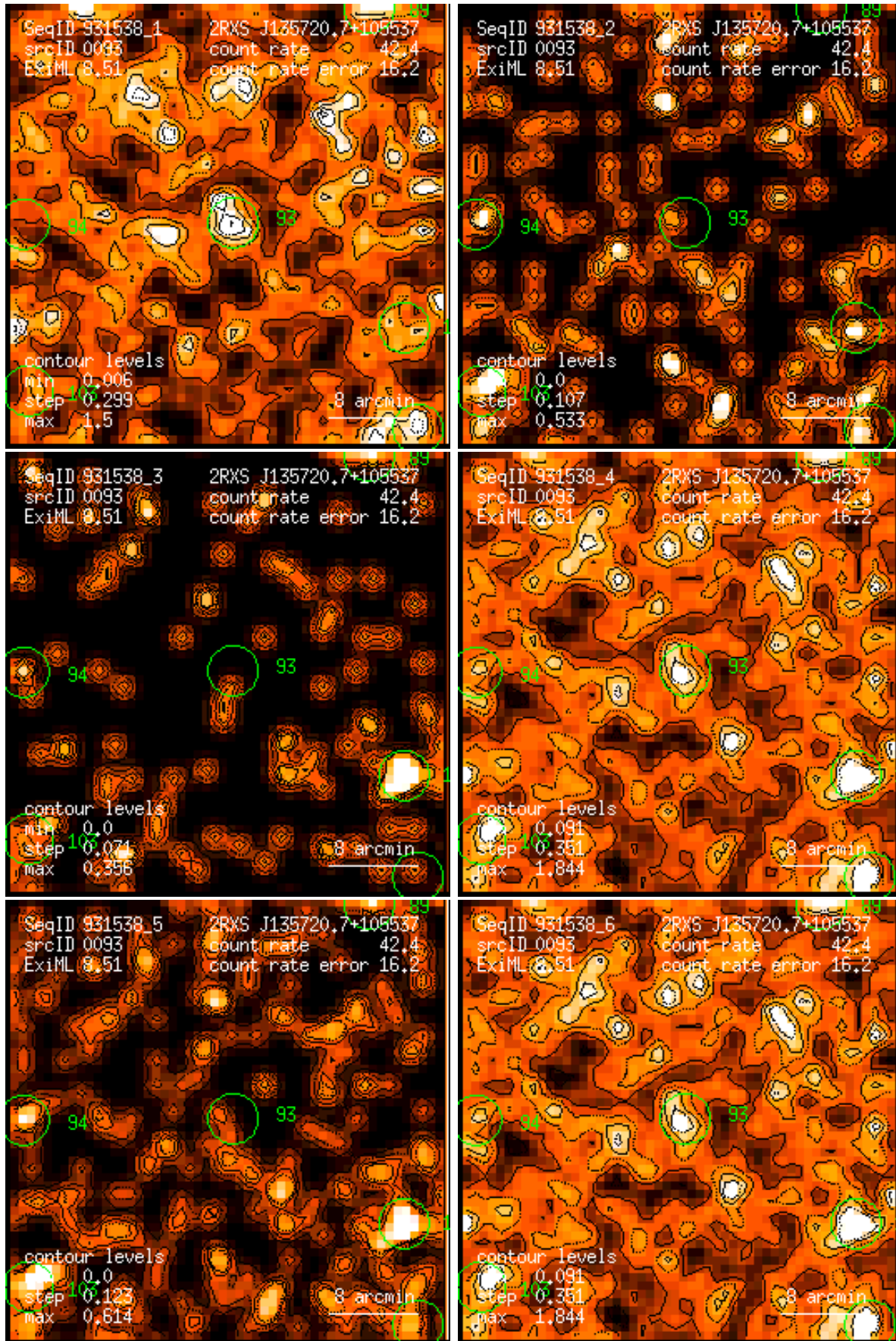
Figure 93: RASS 931538: detection 0093: band rate images, Gaussian filter: (1) PSPC channels 11 – 41, (2) 52 – 90, (3) 91 – 201, (4) 11 – 235, (5) 52 – 201, (6) 11 – 201. Broad band rates in counts/ks. Band rate contour levels in counts/ks/arcmin 2 .
