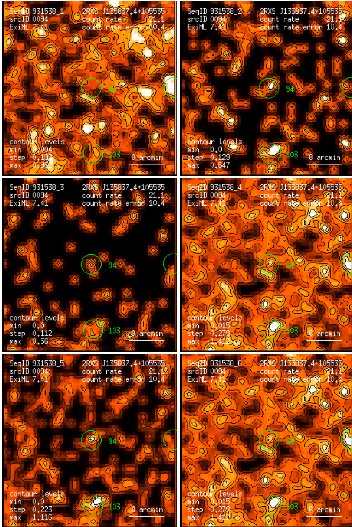
Figure 94: RASS 931538: detection 0094: band rate images, Gaussian filter: (1) PSPC channels 11 – 41, (2) 52 – 90, (3) 91 – 201, (4) 11 – 235, (5) 52 – 201, (6) 11 – 201. Broad band rates in counts/ks. Band rate contour levels in counts/ks/arcmin 2 .
